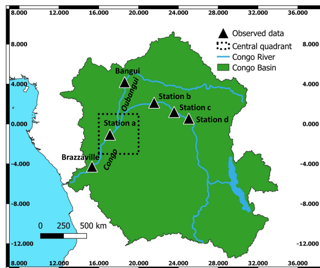
Figure 1. Extent of the Congo Basin, central quadrant of the Cuvette Centrale, and locations of sampling stations used for validation (of DOC, discharge, and partial pressure of \text{CO}_2 ) along the Congo and Oubangui River (in italics).
