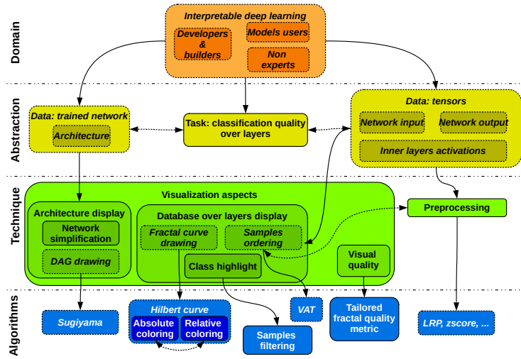
Fig. 1. Nested blocks and guidelines [25] representation of the proposed method. Dotted italic blocks corresponds to existing ones; plain straight blocks are defined in the work.
