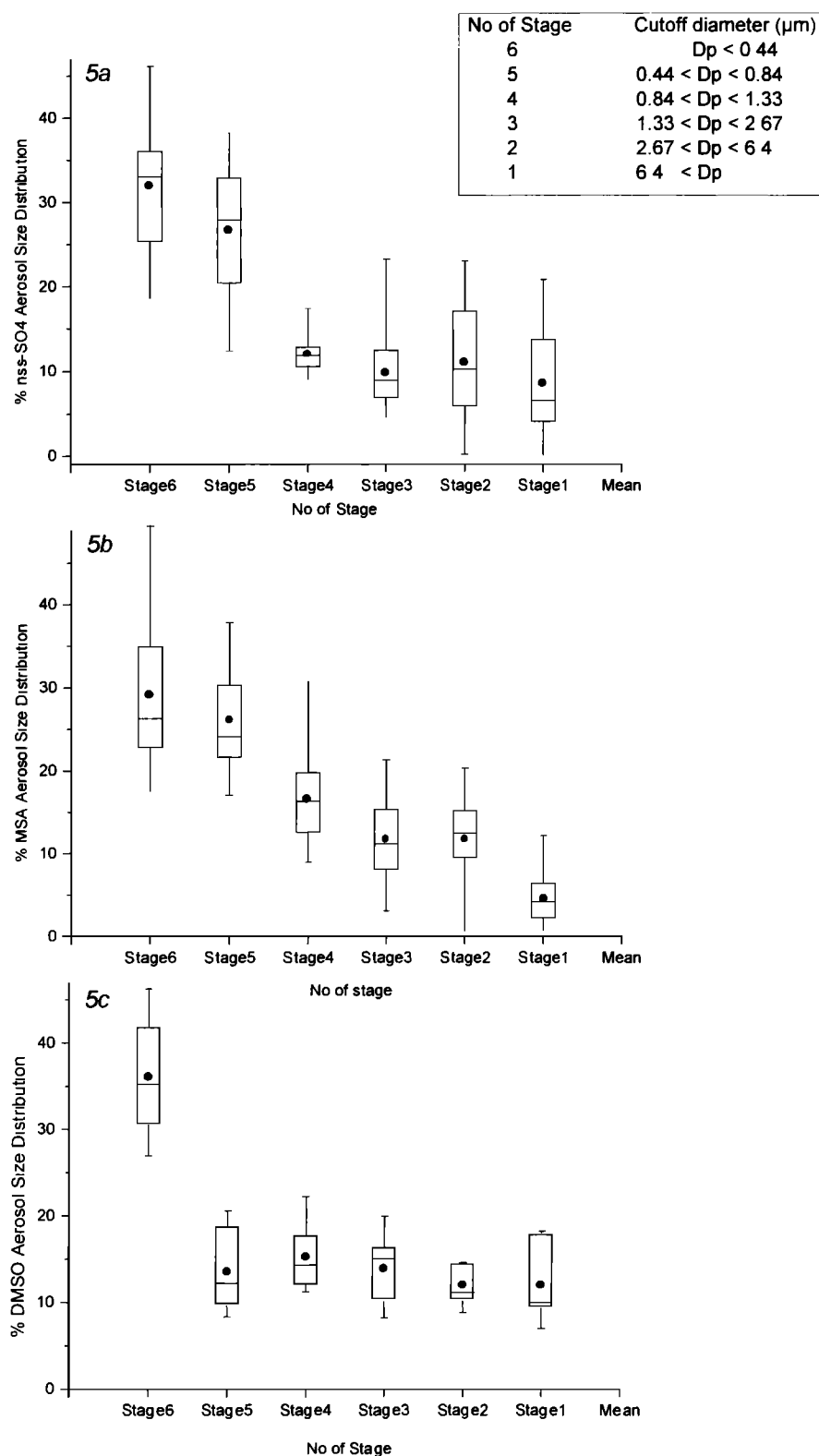
Figure 5. Size fractionation of (a) nss-SO 4 , (b) MSA, and (c) DMSO as a function of diameter during the cruise. The box plots contain the 10 th , 25 th , 50 th , 75 th and 90 th percentiles. The square inside the box plots corresponds to the mean value.
