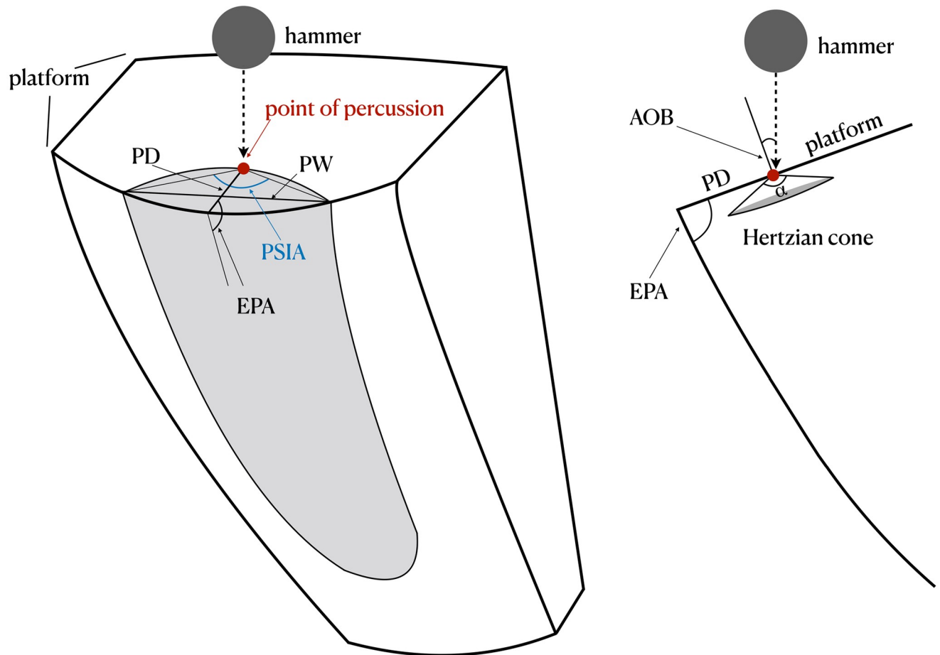
Fig 1. Illustration of several flake attributes discussed here. On the left is a schematic semispherical core used in the Dibble and colleagues glass experiments. On right is a schematic profile of the core through the point of percussion.
