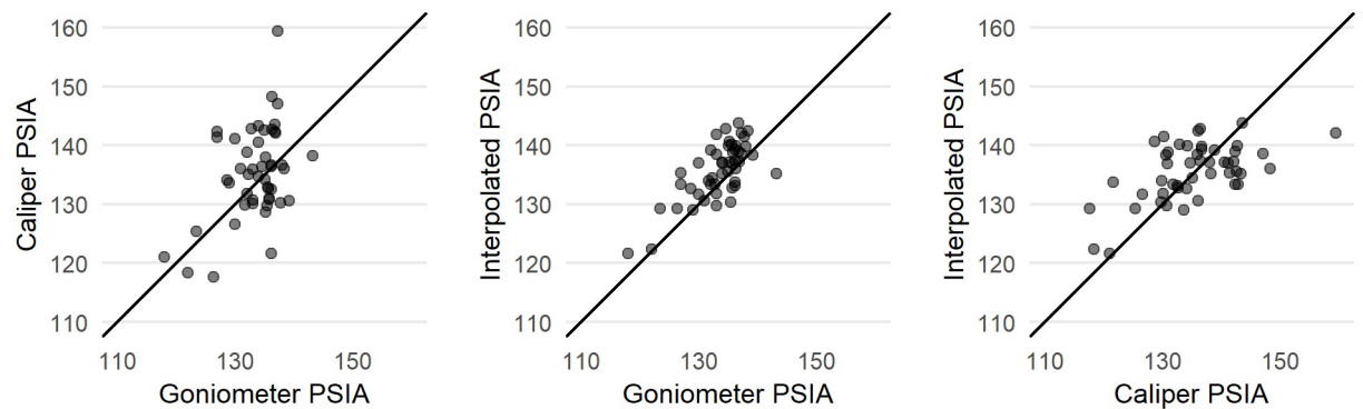
Fig 7. A comparison of the estimated platform surface interior angle, this same angle as calculated from caliper measurements, and this same angle measured with a goniometer. All measures are in degrees.
