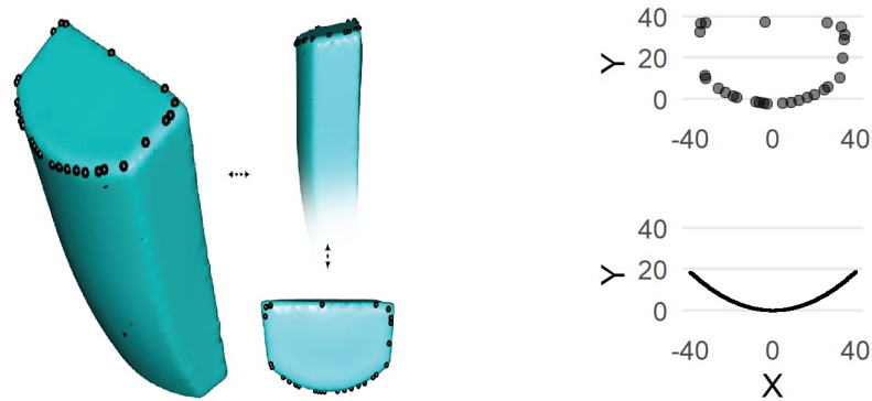
Fig 2. Left, an example of a semispherical glass core from the Dibble and colleagues experiments with landmarks on the platform outline. Above right, those same landmarks plotted in XY space. Below right, the core edge after fitting a polynomial curve to the XY landmarks.
