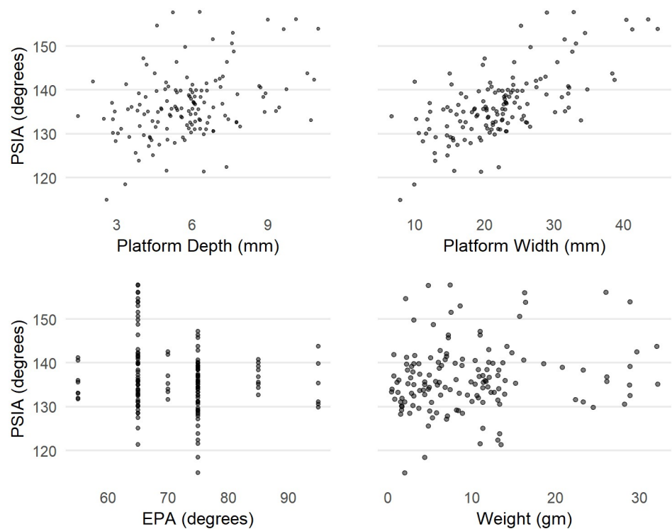
Fig 4. PW, PD, EPA and weight against the estimated PSIA based on the Dibble glass flakes.
