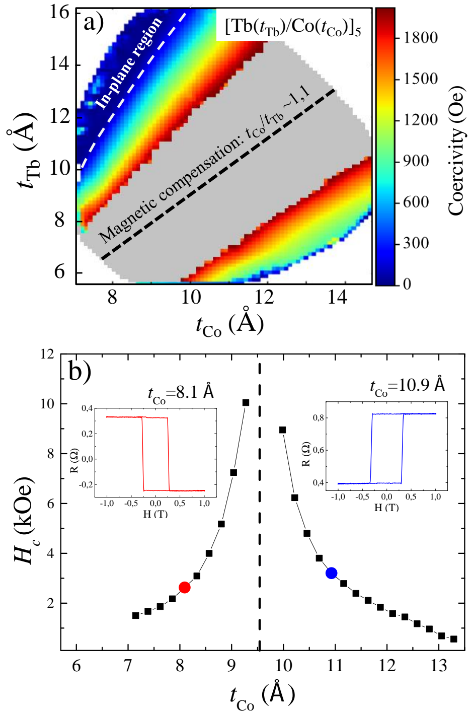
Figure 1. (a) Coercive field map of [\text{Tb}(t_{\text{Tb}})/\text{Co}(t_{\text{Co}})]_5 . The coercive field values were obtained from the M(H) loops measured with H applied perpendicular to the plane of the film. The superimposed gray region in the center indicates the region in which H was not sufficient to saturate the stack. The black dashed line schematically represents the thickness values of Tb and Co for which the coercive field diverges i.e. where magnetic compensation occurs at room temperature. (b) Coercive field of [\text{Tb}/\text{Co}]_5 multilayer as a function of Co thickness t_{\text{Co}} : 7 - 13 Å with the thickness of the Tb layers fixed at t_{\text{Tb}} = 10 Å. Insets: R(H) for t_{\text{Co}} = 8.1 Å and t_{\text{Co}} = 10.9 Å as indicated.
