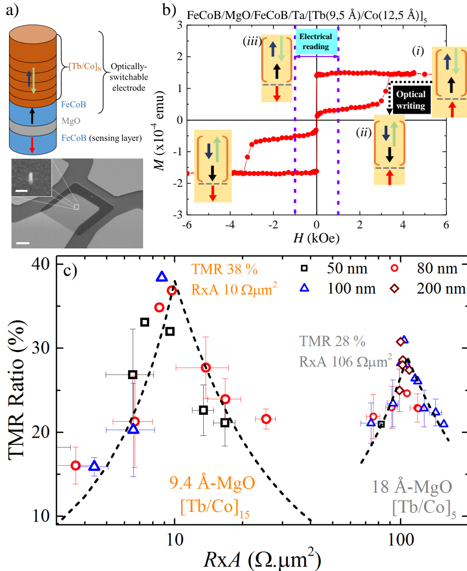
Figure 4. a) Top: Schematic of the MTJ studied. The MTJ consists of an optically-switchable storage layer CoFeB ( 13 \text{ \AA} )/Ta/ [\text{Tb}/\text{Co}]_N and a CoFeB free layer, separated by a MgO tunnel barrier. Bottom: SEM Image of the 50 nm patterned MTJ in an intermediate step of the nanofabrication process. (scale bar: 4 \mu\text{m} ). Inset: Zoom of the capping layer of the 50 nm-junction before the deposition of the upper electrical contact (scale bar: 100 nm) b) Out-of-plane M(H) curve measured for the MTJ with the stack [\text{Tb}/\text{Co}]_5 . Insets: illustrations of the 4 magnetic states of the MTJ indicating the stages intended for optical writing (state (i) to state (ii)) and electrical readout (state (i) to state (iii)). c) TMR vs RxA of nano-patterned junctions for stacks with different repetition numbers N of the [\text{Tb}/\text{Co}]_N stacks as indicated, with 9.4 \text{ \AA} and 18 \text{ \AA} MgO barriers. The dispersion in the TMR and RxA as calculated from shunt and series resistance models (dashed lines) are also shown. The wafer-level TMR potential for optimal processing is 38% and 28% respectively.
