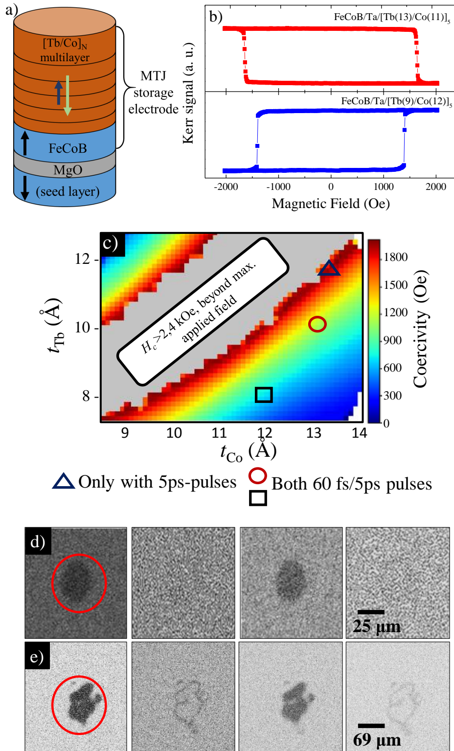
Figure 3. a) Structure of half-MTJ stack used to optimize the magnetic coupling between the [Tb(10 Å)/Co(12 Å)] 5 multilayer and the CoFeB electrode. b) Hysteresis loop of the CoFeB/Ta/[Tb( t Tb )/Co( t Co )] 5 stack measured on opposite sides of the compensation region. c) Coercivity map of the half-MTJ along the Tb and Co thickness wedges. The regions enclosed by the symbols indicate the three regions of the CoFeB/Ta/[Tb( t Tb )/Co( t Co )] 5 structure in which all-optical switching was achieved using different pulse durations: \Delta : [Tb(11 Å)/Co(13 Å)] 5 , \circ : [Tb(10 Å)/Co(13 Å)] 5 and \square : [Tb(8 Å)/Co(12 Å)] 5 as indicated. d-e) Background-corrected magneto-optical images demonstrating successful single-shot all-optical switching of magnetization in the CoFeB/Ta/[Tb(10 Å)/Co(13 Å)] 5 stack using d) ps- and e) fs-long laser pulses in with an incident fluence of 4.7 mJ/cm 2 and 3.5 mJ/cm 2 respectively.
