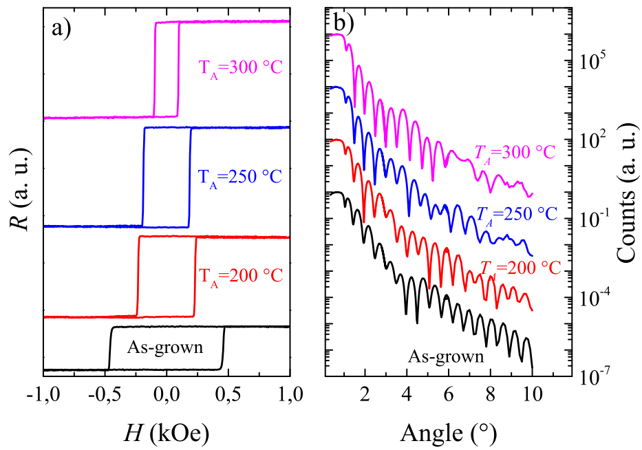
Figure 2. (a) R(H) obtained from EHE experiments and b) x-ray reflectivity measurements of [\text{Tb}(10 \text{ \AA})/\text{Co}(12 \text{ \AA})]_5 samples as-deposited and annealed at temperatures T_A = 200, 250 and 300^\circ\text{C} as indicated.
