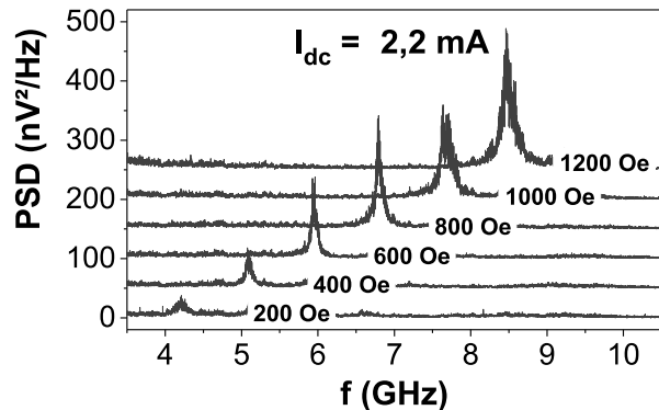
Figure 10: Spectrum of the RF response to a DC current, with in-plane field
