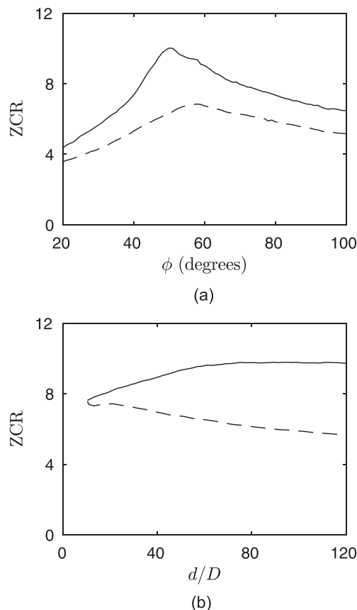
FIG. 9. Mean number of zero-crossings during a time t = D/u_j on the circular (a) and line (b) arrays for linear (solid lines) and nonlinear (dashed lines) propagations.
