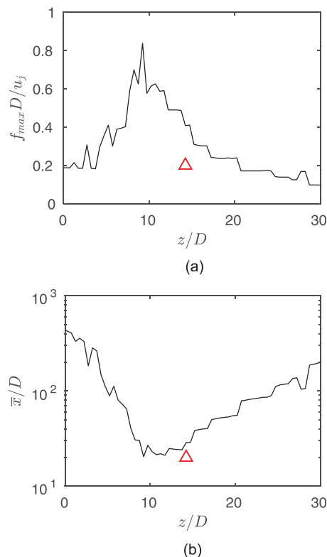
FIG. 14. (Color online) Axial variations at r = 7.5D of the peak Strouhal number of the pressure fluctuations (a) and shock formation distance (b). The red triangles indicate the location of peak acoustic levels.
