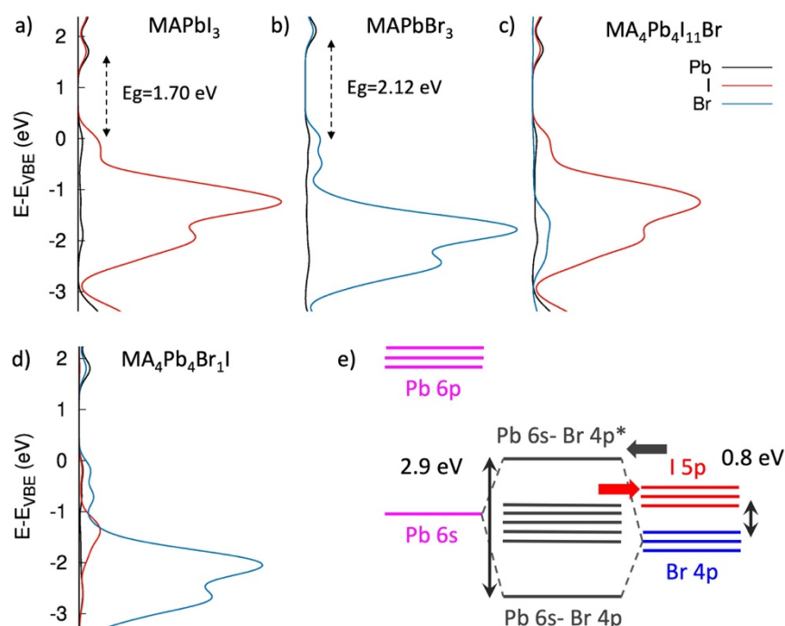
Figure 1. a-b) atomic projected Density of States (pDOS) for pure halide MAPbI 3 (a), MAPbBr 3 (b) compounds, in their corresponding tetragonal phase. c-d) pDOS for mixed halide MA 4 Pb 4 I 11 Br (c) and MA 4 Pb 4 Br 1 I (d) compounds. Contributions from lead, iodine and bromine atoms are reported in black, red and blue, respectively. e) schematics of the hybridization of the atomic orbitals for the valence band, as composed by combination of s-states of lead (magenta) and p-states of the iodine (red) and bromine (blue), along with indication of the valence bandwidth and difference in atomic site energies for Br 4p and I 5p states.
