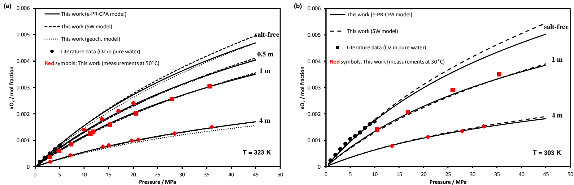
Figure 8 : O_2+H_2O+NaCl system : Prediction of O_2 solubility at different NaCl molality m ( mol/kg_w ) by e-PR-CPA (solid line), SW (dashed line) and geochemical (dotted line) models. The black symbols are the literature data ((a) : 34 , (b) : 35 ), and the red symbols are the measured data (Table 3).
