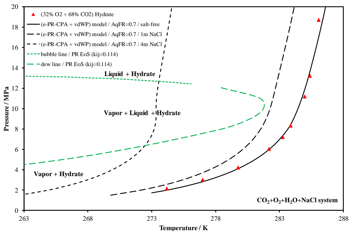
Figure 11: Hydrate dissociation conditions of the \text{CO}_2+\text{O}_2+\text{H}_2\text{O}+(\text{NaCl}) quaternary system: Prediction of the effect of NaCl concentration (from salt-free to 4m) on the mixed-gas hydrate system (32% \text{O}_2 , at fixed aqueous fraction AqFr=0.7) using the (e-PR-CPA + vdWP) model. The bubble and dew lines are determined by the PR EoS.
