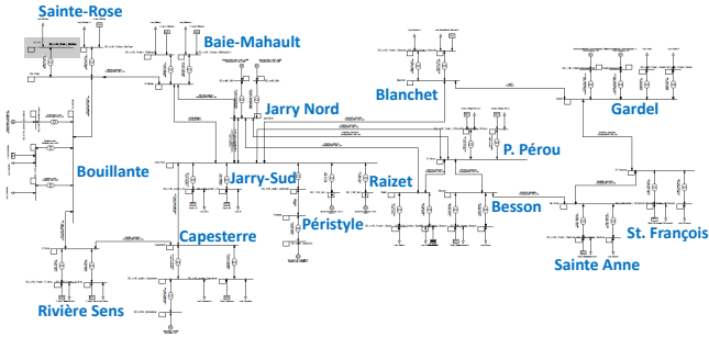
Fig. 2. Guadeloupe island electrical model.
