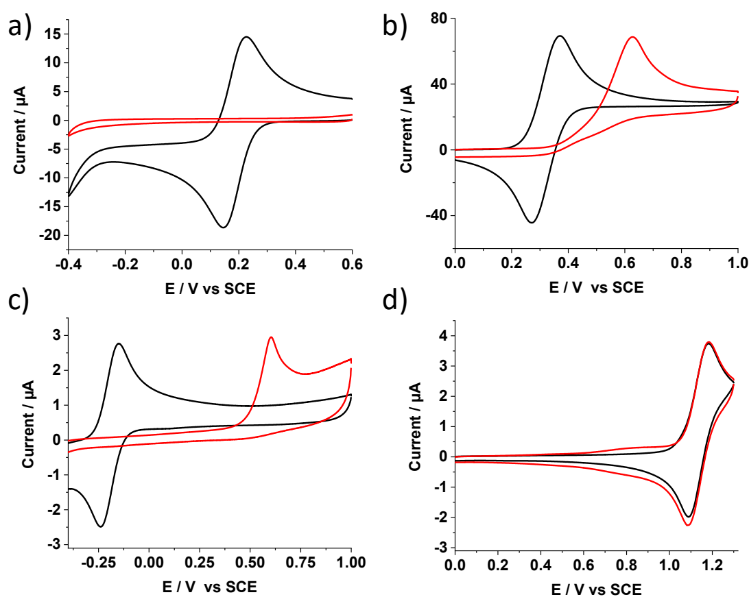
Figure 3. Electrochemical response of bare (black) and modified (red) electrodes in various redox probe solutions: (a) \text{K}_3\text{Fe}(\text{CN})_6 1 mM; (b) ferrocene 1 mM; (c) decamethylferrocene 1 mM; (d) thianthrene 1 mM with 0.1 M \text{LiClO}_4 in ACN solution.
