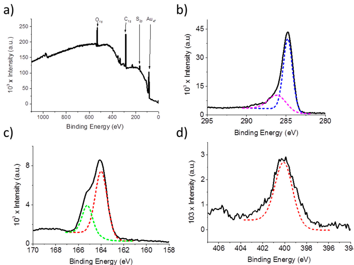
Figure 5. High-resolution XPS spectra of SNS-An modified gold surface. (a) XPS survey spectra of gold modified electrode. (b) \text{C}_{1s} spectra. (c) \text{S}_{2p} spectra. (d) \text{N}_{1s} spectra.
