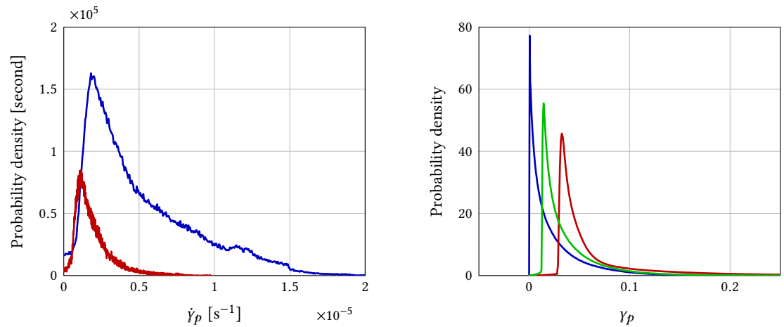
Figure 19 Field histograms. (a) Equivalent plastic strain rate in the binder at 75 °C during heating (blue) and cooling (red) with T_0 = 20 °C and T_{\max} = 80 °C. (b) Cumulated equivalent plastic strain during heating at 80 °C (blue) and during cooling at 20 °C (green) and -60 °C (red).
