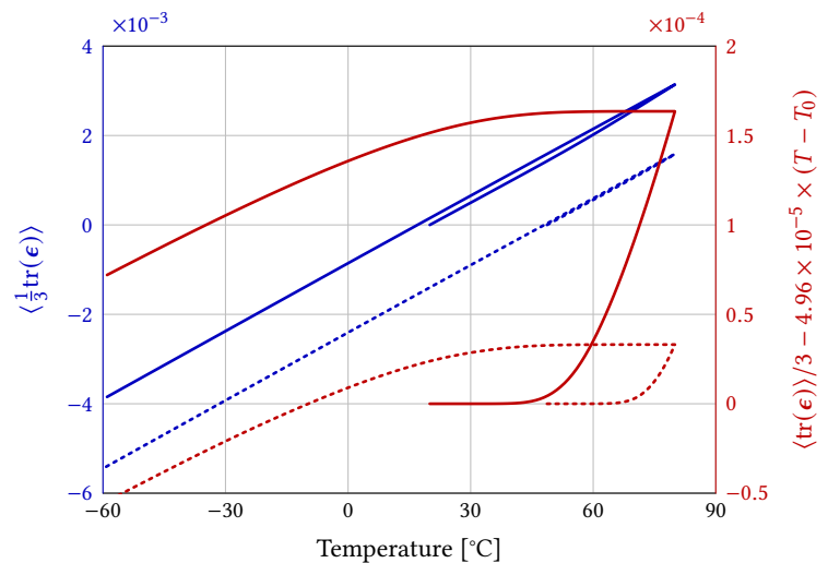
Figure 16 Computed thermal cycles from the stress-free state at T_0 = 20^\circ\text{C} (solid) and T_0 = 48.7^\circ\text{C} (dotted) to T_{\max} = 80^\circ\text{C} , and cooling to T_f = -60^\circ\text{C} . Left vertical axis: thermograms. Right vertical axis: nonlinear parts.
