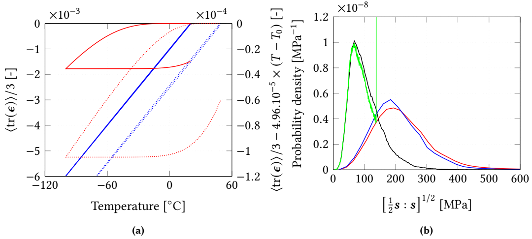
Figure 14: Cooling from T_0 down to -100^\circ\text{C} and heating back. (a) Thermogram (blue, left vertical axis), and departure from initial linear slope (red, right vertical axis). Solid: T_0 = 20^\circ\text{C} , dotted: T_0 = 48.7^\circ\text{C} . (b) Case T_0 = 48.7^\circ\text{C} . Histograms of equivalent stress at -100^\circ\text{C} in the grains (blue and red) and the binder (green and black) for purely elastic cooling (blue and black) and for elasto-plastic cooling (red and green).
