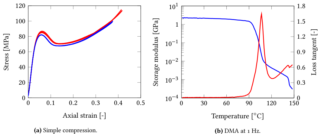
Figure 13: (a) Binder uniaxial compression response at 10^{-4} (blue) and 10^{-3} \text{ s}^{-1} (red) at room temperature. (b) Storage modulus (blue, left vertical axis) and loss tangent (red, right vertical axis) measured at 1 Hz by Dynamic Mechanical Analysis (DMA).
