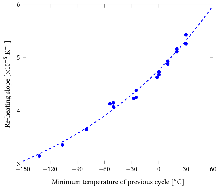
Figure 9: Slopes of the linear parts of heating phases of the experiments illustrated in Fig. 8 versus the minimum temperature of the preceding thermal cycle, regardless of the thermal history of each experiment. Dashed curve: Eqn. (1).
