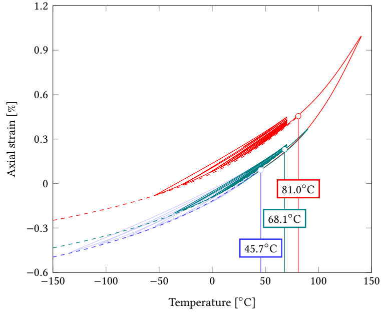
Figure 8: Result of cold cycles after an excursion at 90°C (green curve) and at 140°C (red curve), compared to the data of Fig. 6 (light blue curve). The open circles indicate the common origin of each experiment. Dashed curves: see text and Eqn. 1.
