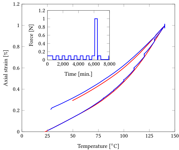
Figure 5: Thermal creep experiment (thin dark blue curve) performed at 80, 90, 100, 110, 120, 130, 140 and 130^{\circ}\text{C} , versus single cycle to 140^{\circ}\text{C} (red curve). Inset: force vs. time.
