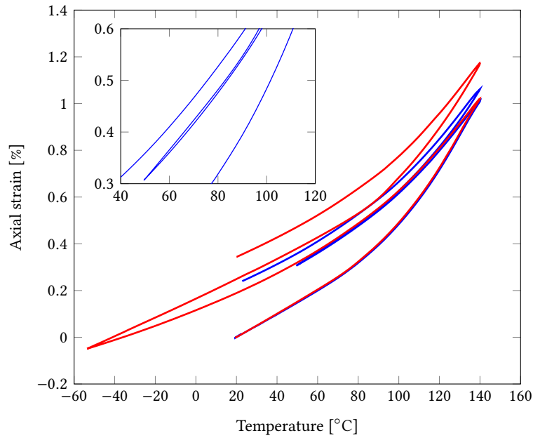
Figure 11: Double hot cycles at 140°C separated by a cold cycle at 50°C (dark blue curve) and at -50°C (red curve). The inset is a magnification of the blue curve, showing that cooling at 50°C is not reversible.
