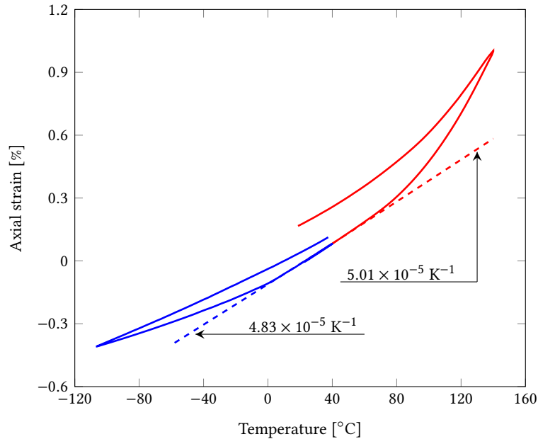
Figure 2: Two cyclic experiments below (blue) and above (red) room temperature.
