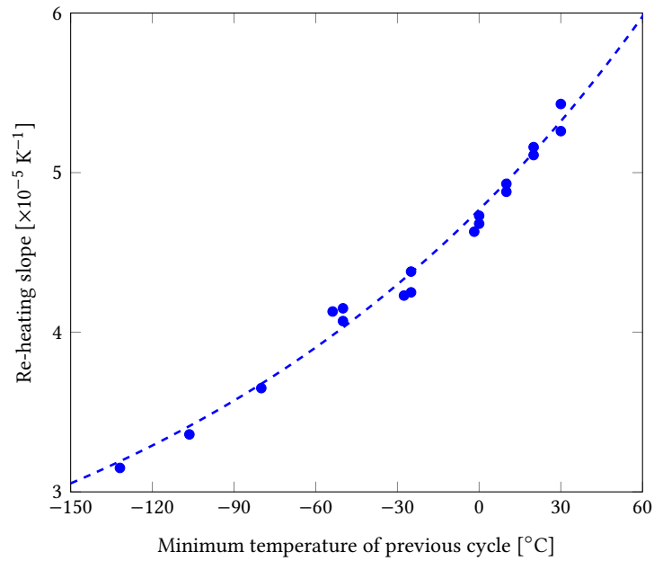
Figure 9: Slopes of the linear parts of heating phases of the experiments illustrated in Fig. 8 versus three minimum temperature of the preceding thermal cycle, regardless of the thermal history of each experiment. Dashed curve: Eqn. (1).
