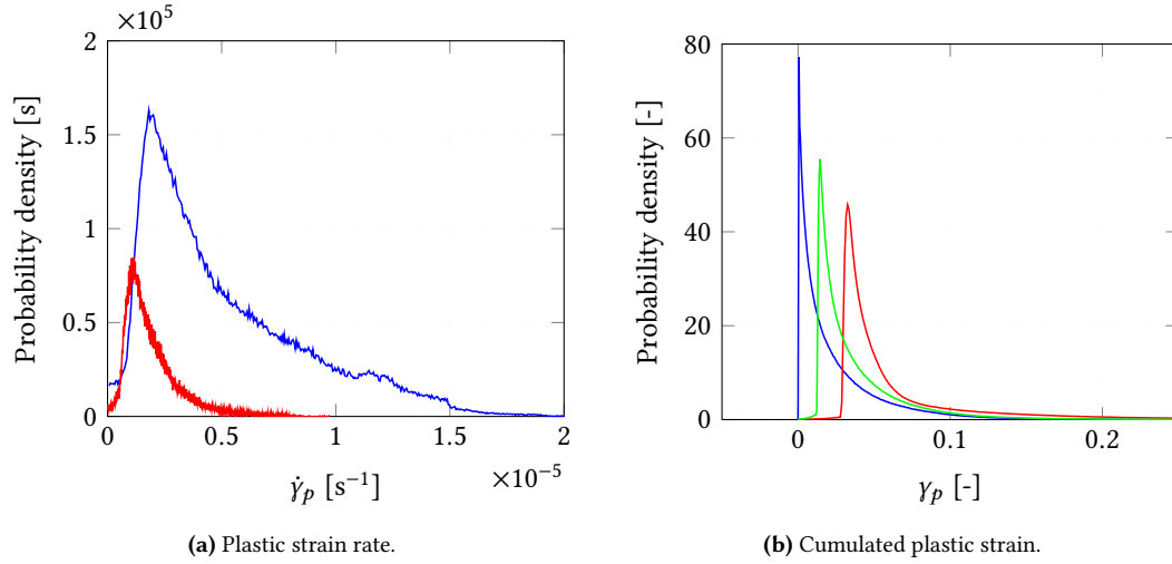
Figure 18: Field histogram for (a) the equivalent plastic strain rate in the binder at 75^\circ\text{C} during heating (blue) and cooling (red). T_0 = 20^\circ\text{C} , T_{\text{max.}} = 80^\circ\text{C} , (b) the cumulated equivalent plastic strain during heating at 80^\circ\text{C} (blue) and during cooling at 20^\circ\text{C} (green) and -60^\circ\text{C} (red).
