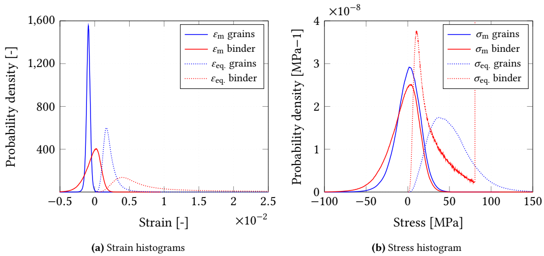
Figure 16: (a) Field histograms for the mean (solid) and von Mises equivalent (dashed) strains in the grains (blue) and in the binder (red), at T = 20^\circ\text{C} , upon heating and cooling, from an initial stress-free state at temperature T = T_0 = 20^\circ\text{C} . (b) Mean (solid) and Von Mises (dashed) stress in the grains (blue) and binder (red).
