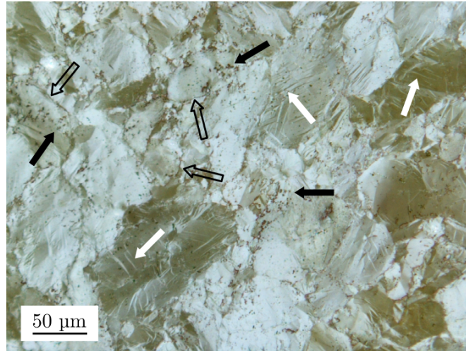
Figure 1: Microstructure of the of the composite (polarized reflected light microscopy). Black arrows: pores and pore clusters. White arrows: probable deformation twins. Open arrows: possible intra-transgranular microcracks.
