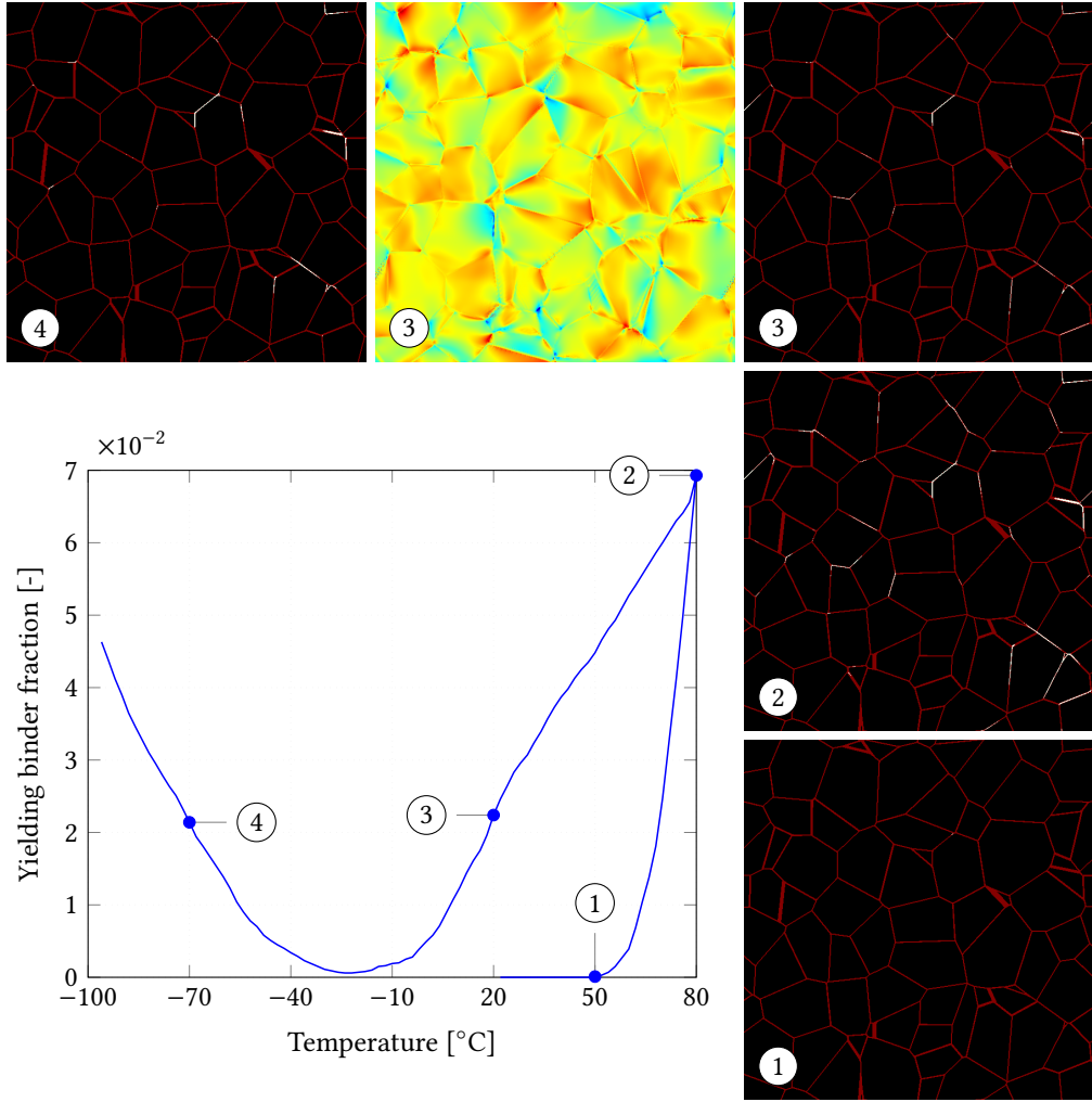
Figure 17: Evolution of the binder fraction experiencing plastic yielding during heating from T_0 = 20 to 80^\circ\text{C} , and cooling to -100^\circ\text{C} . Each blue dot corresponds to a FFT map of yielding binder (grains in black), from bottom right to top left, during heating at 50 (onset of yielding) and 80^\circ\text{C} , and during cooling at 20 and -70^\circ\text{C} . White: yielding. Red: no yielding. The colored image is a map of residual mean stresses back at 20^\circ\text{C} . Min.: -56 (blue) MPa. Max.: 34 MPa (red).
