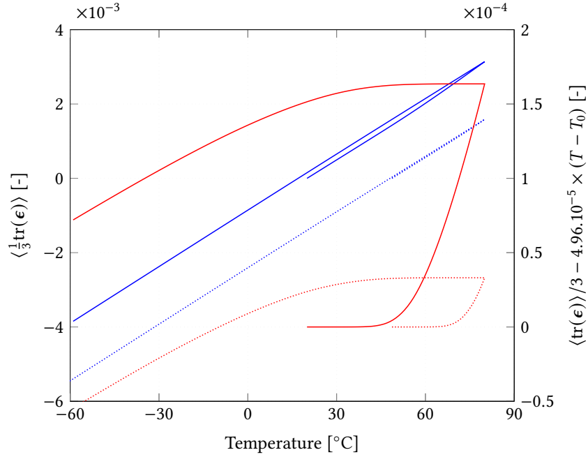
Figure 15: Computed thermal cycles from the stress-free state at T_0 = 20^\circ\text{C} (solid) and T_0 = 48.7^\circ\text{C} (dotted) to T_{\text{max.}} = 80^\circ\text{C} , and cooling to T_f = -60^\circ\text{C} . Blue: thermograms. Red: nonlinear parts.
