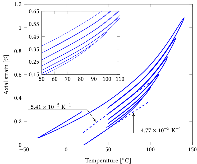
Figure 4: Cycles from 50^{\circ}\text{C} to maximum temperatures of 90, 100, 110, 120, 130, 140 and -30^{\circ}\text{C} . The inset is an enlargement to show the details in the glassy domain and just above.
