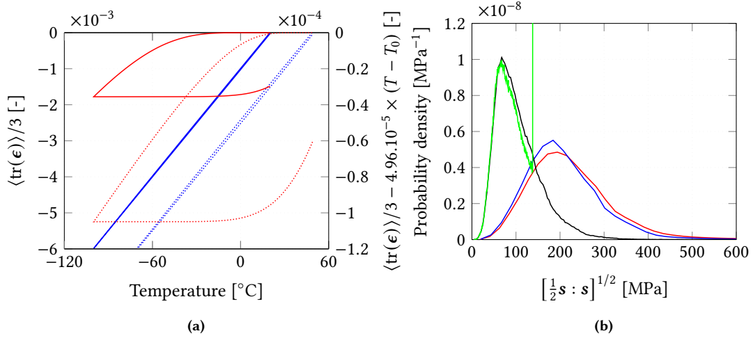
Figure 14: Cooling from T_0 down to -100^\circ\text{C} and heating back. (a) Thermogram (blue), and departure from initial linear slope (red). Solid: T_0 = 20^\circ\text{C} , dotted: T_0 = 48.7^\circ\text{C} . (b) Case T_0 = 48.7^\circ\text{C} . Histograms of equivalent stress at -100^\circ\text{C} in the grains (blue and red) and the binder (green and black) for purely elastic cooling (blue and black) and for elasto-plastic cooling (red and green).
