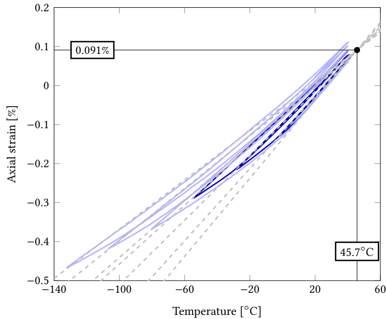
Figure 7: Common origin of the linear parts of each re-heating phases, found by optimization.
