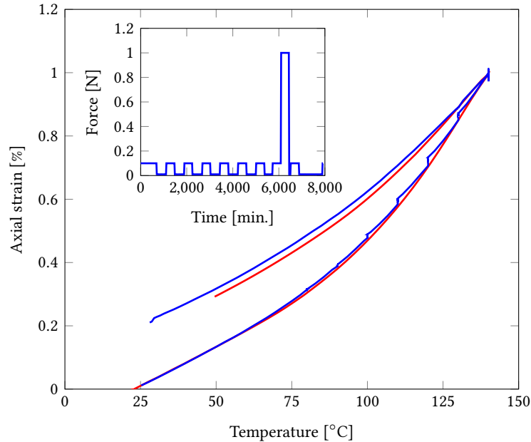
Figure 5: Thermal creep experiment (thin dark blue curve) performed at 80, 90, 100, 110, 120, 130, 140 and 130°C, versus single cycle to 140°C (red curve). Inset: force vs. time.
