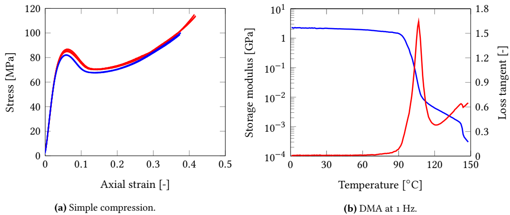
Figure 13: (a) Binder uniaxial compression response at 10^{-4} (blue) and 10^{-3} \text{ s}^{-1} (red) at room temperature. (b) Storage modulus and loss tangent measured at 1 Hz by Dynamic Mechanical Analysis (DMA).
