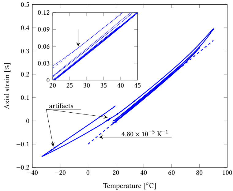
Figure 3: Cycles from ambient temperature to maximum temperatures of 40, 60, 70, 80, 90 and -30^{\circ}\text{C} . The cycles to 40, 60 and 70^{\circ}\text{C} are reversible. The inset is an enlargement near ambient temperature. The dashed lines are the linear approximations of the last two cooling phases, and the arrow marks the point from which the last cooling departs from linearity, indicating the beginning of irreversible behavior.
