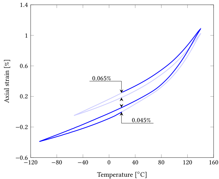
Figure 10: Hot cycles with (dark bleu curve) and without (light blue curve) pre-cooling at -106^{\circ}\text{C} .
