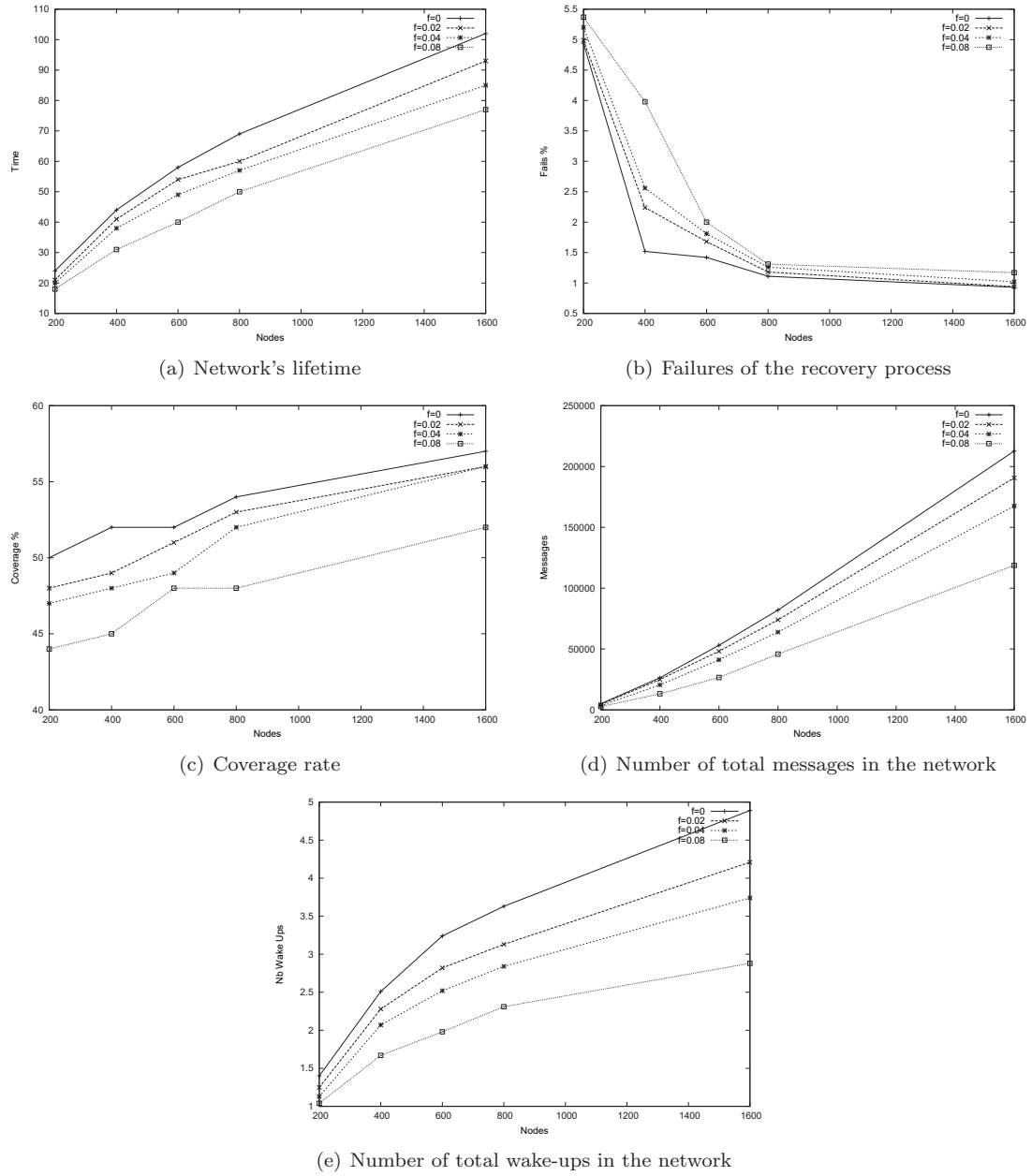
FIGURE 4. Performance evaluation with average (1x) wake up rate.
