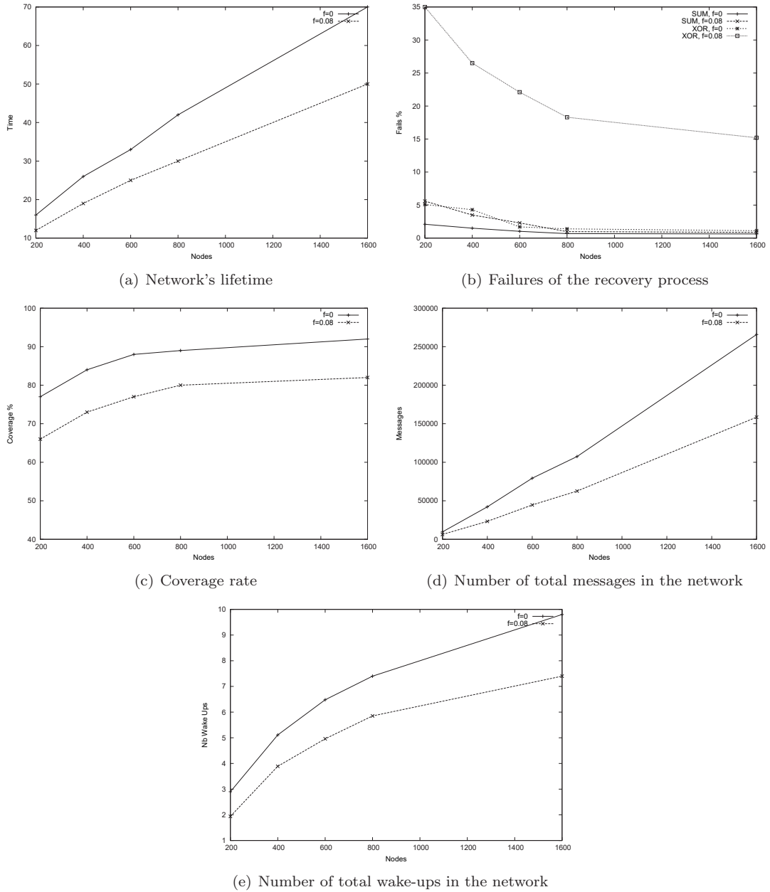
FIGURE 5. Performance evaluation with high (4x) wake up rate.
