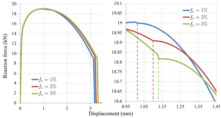
Figure 34: Notched axisymmetric specimen - RF vs Displacement response for different critical porosities f_c (left) and Zoom-in the region of apparent inflection (right)
