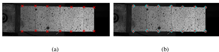
Fig. 20 (a) Fiducials (in red crosses) on one of the image pair on the calibration target and (b) estimated 2D positions (in cyan asterisks) of these points through initial projection matrix obtained with an SVD pre-calibration, along with manually clicked points (in red crosses).
