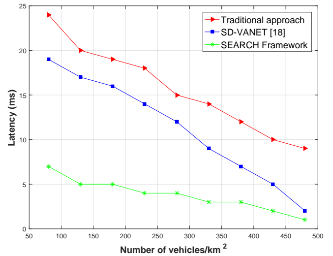
(b) Latency vs. Density of vehicles.
