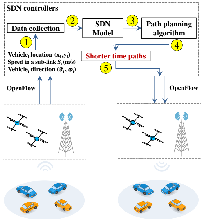
Fig. 2: Key functionalities and components of SEARCH.
