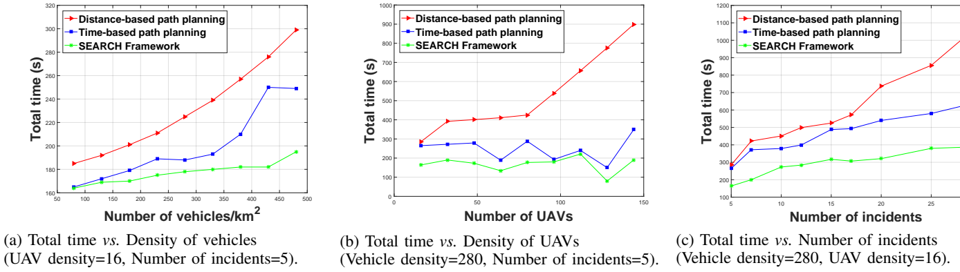
Fig. 9: Simulation results of journey time of SEARCH.
