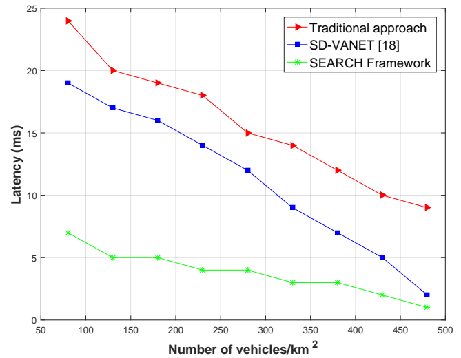
(b) Latency vs. Density of vehicles.
