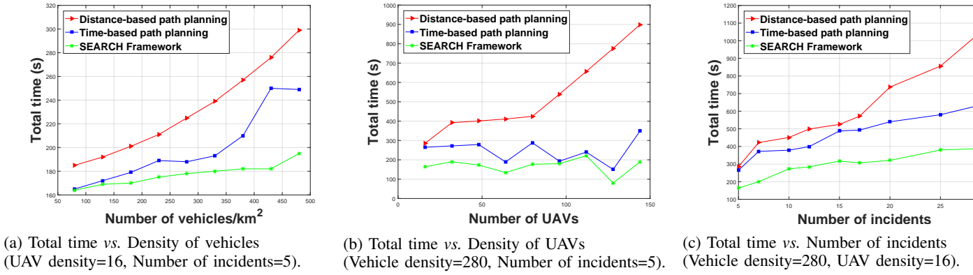
Fig. 9: Simulation results of journey time of SEARCH.
