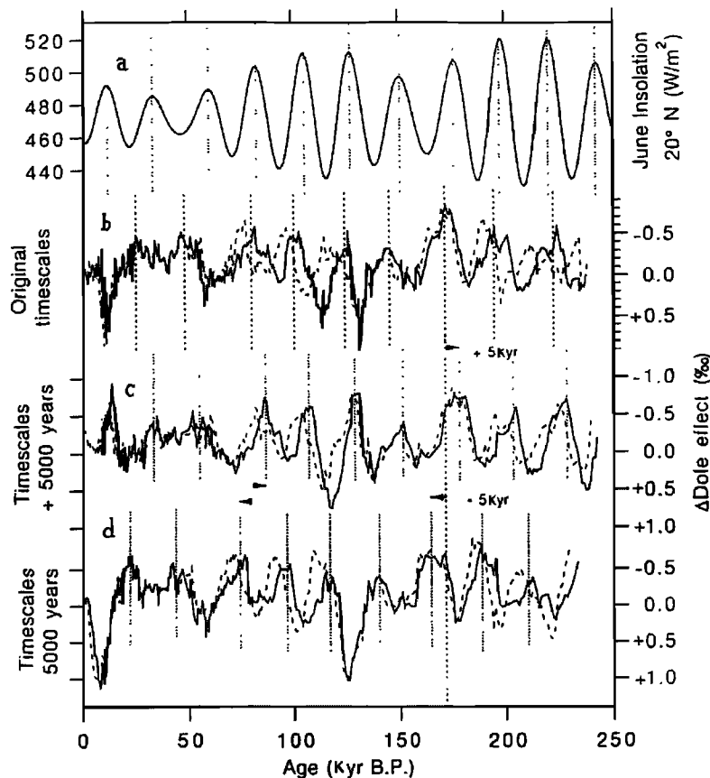
Figure 3. (a) The summer solstice insolation at 20°N [Berger, 1978]. The sensitivity of the \Delta Dole record to changes in timescales, this record being calculated (b) with the EGTmod timescale [Jouzel et al. , 1996] and the ICT timescale (dashed line), (c) in adding 5 kyr to the Vostok timescales (see text), and (d) in subtracting 5 kyr.
