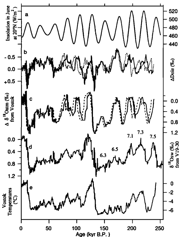
Figure 1. Variations with time of (a) the summer solstice insolation (June 21) at 20°N [Berger, 1978], (b) the Dole effect as calculated from \delta^{18}\text{O}_{\text{atm}} and \delta^{18}\text{O}_{\text{sw}} records, (c) the \delta^{18}\text{O}_{\text{atm}} record from gas analysis of the Vostok ice core dated with gas age timescales, (d) the \delta^{18}\text{O}_{\text{sw}} record from the V19-30 core modified as described in the text, and (e) the mean atmospheric temperature at the Vostok site (Antarctica) (EGTmod timescale) as deduced from the ice deuterium content [Jouzel et al. , 1996]. The solid and dashed lines in figures 1b and 1c are for the Dole record calculated using the \delta^{18}\text{O}_{\text{atm}} record dated with the extended glaciological timescale modified (EGTmod) and the isotopic correlation timescale (ICT) respectively. The annotations in figure 1d give the different stages as defined by Martinson et al. [1987].
