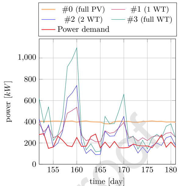
Figure 8: Renewable power production in June 2004 for each possible configuration found by the sizing algorithm to meet the data center demand.
