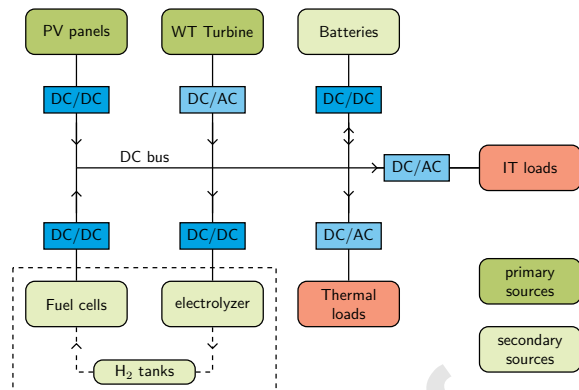
Figure 1: Electrical architecture of DATAZERO. Dark green boxes indicate primary energy sources, secondary sources are shaded in light green (source: Robin Roche).
