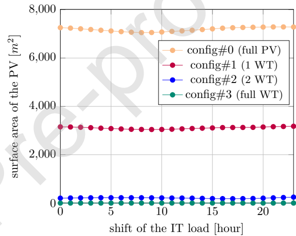
Figure 11: Evolution of the surface area of the photovoltaic panels as a function of the shift of the IT load.
