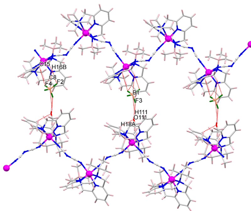
Figure 7. Packing diagram of 1 at 296 K showing the supramolecular double chain (bottom) formed by several C–H⋯F and C⋯F (red dotted lines) interactions (Co, pink; C, gray; N, blue; B, light pink; F, green).
