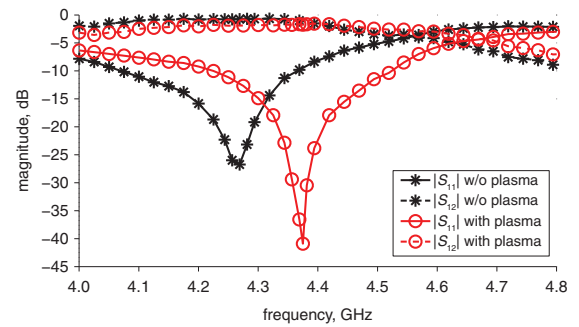
Fig. 3 Measured S parameters in argon at P = 1 Torr without plasma ( I_{\text{DC}} = 0 mA) and with plasma ( I_{\text{DC}} = 62 mA)
