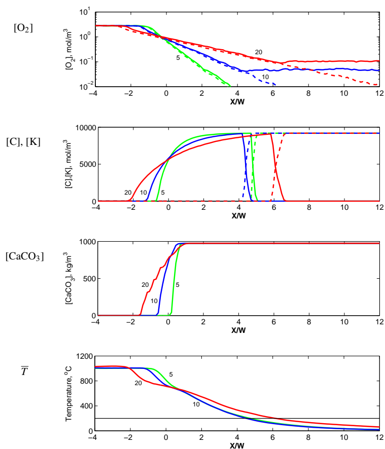
Fig. 4 Profiles of [O_2] , of [C] (—) and [K] (---), of [CaCO_3] and of \bar{T}_s , for {OCP} with \Delta = 0.38 and Pe=5, 10 et 20 . [O_2] is also shown for {O}(-.-). Distances are measured relative to the front position X_F .
