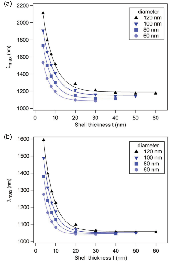
FIG. 3. (Color online) Calculated fundamental wavelength \lambda_{\max} of the maximum of the SH (a) dipolar and (b) quadrupolar emission modes for a silica core-gold shell nanoparticle in water as a function of the shell thickness t for four nanoshell diameters. Solid lines correspond to fits with exponential functions.
