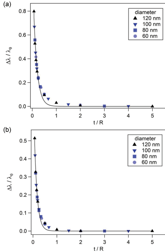
FIG. 4. (Color online) Fractional shift \Delta\lambda/\lambda_0 of the SH (a) dipolar and (b) quadrupolar emission modes for a silica core-gold shell nanoparticle in water with respect to that of a solid gold nanosphere with the same size, as a function of the ratio of the shell thickness to the core radius t/R for four different diameters. The solid lines correspond to fits with exponential functions.
