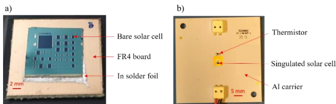
Fig. 5. Photographs of a) a sample with 35 bare cells assembled on a FR4 board for the PSSAT and b) a 0.076-mm 2 singulated cell on a Al carrier for the ASSAT.
