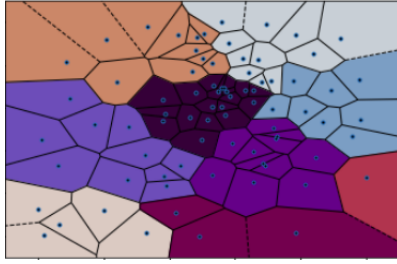
(a) 2D Euclidean K-means. Utilization: 1.13, Cost: 0.86
