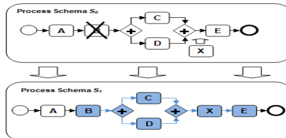
Fig. 3. Deletion of activity 'B' and addition of activity 'X'.
