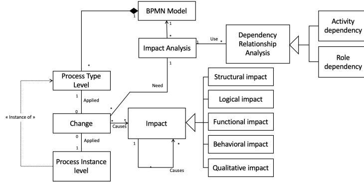
Fig. 2. Meta-model of change impact analysis.
