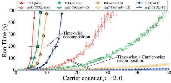
Fig. 6. Models computational complexity related to user and sub-carrier count. In this figure the user to sub-carrier ratio is kept constant to avoid effects highlighted in Fig. 4. ( N_{tests} = 50 )
