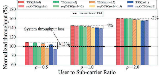
Fig. 4. Performance of the different models solution according to the user to sub-carrier ratio. Sub-carrier count is kept constant ( N_{carriers} = 8 ) so that physical capacity is kept constant, while the user diversity varies with user count ( N_{users} \in \{4, 8, 16\} ). ( N_{tests} = 200 )
