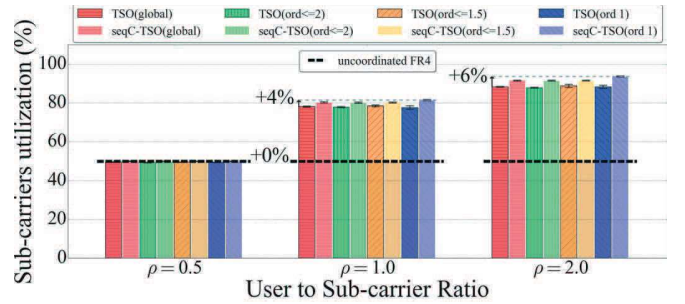
Fig. 5. Sub-carriers utilization according to the user to sub-carrier ratio.
