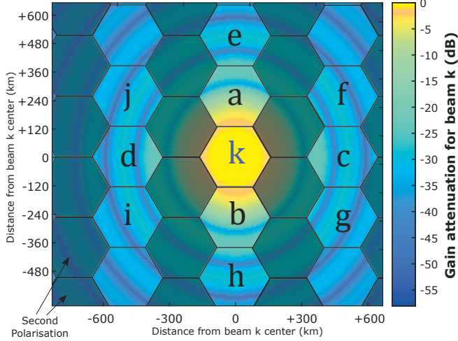
Fig. 3. Interference power generated by users located in beams of the same polarization as the reference beam k
