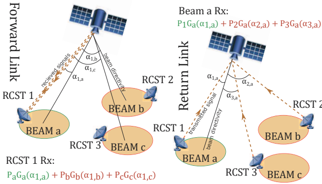
Fig. 1. Interference in the Forward Link and Return Link
