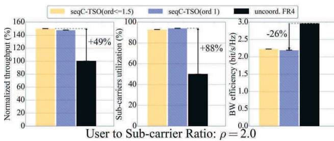
Fig. 7. Results for a larger scenario (90 beams, 30 carriers, 60 users per beam), comparing seqC-TSO(ord 1) , seqC-TSO(ord \leq 1.5) and the reference FR4 scheme. The Bandwidth efficiency is also considered here. ( N_{tests} = 100 )
