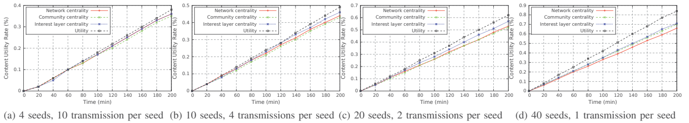
Fig. 4. Content utility rate in terms of seeds number and number of transmission per seed
