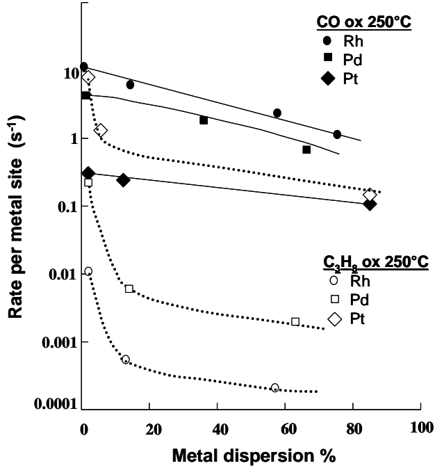
Fig. 5. Effect of metal dispersion on turnover frequencies in CO and propane oxidation (M/Al 2 O 3 catalysts). Adapted from the data of Yu Yao [53,54].
