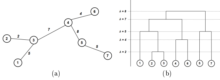
Fig. 1. (a) Example of minimum spanning tree and (b) associated dendrogram.
