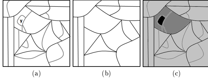
Fig. 2. (min, max)-eigenfunction at point y \in X and eigenvalue \lambda : (a) and (b) depict two partitions of a discrete ultrametric space at levels \lambda and \lambda + 1 ; (c) eigenfunction \phi_\lambda^y(x) . Black corresponds to \lambda .
