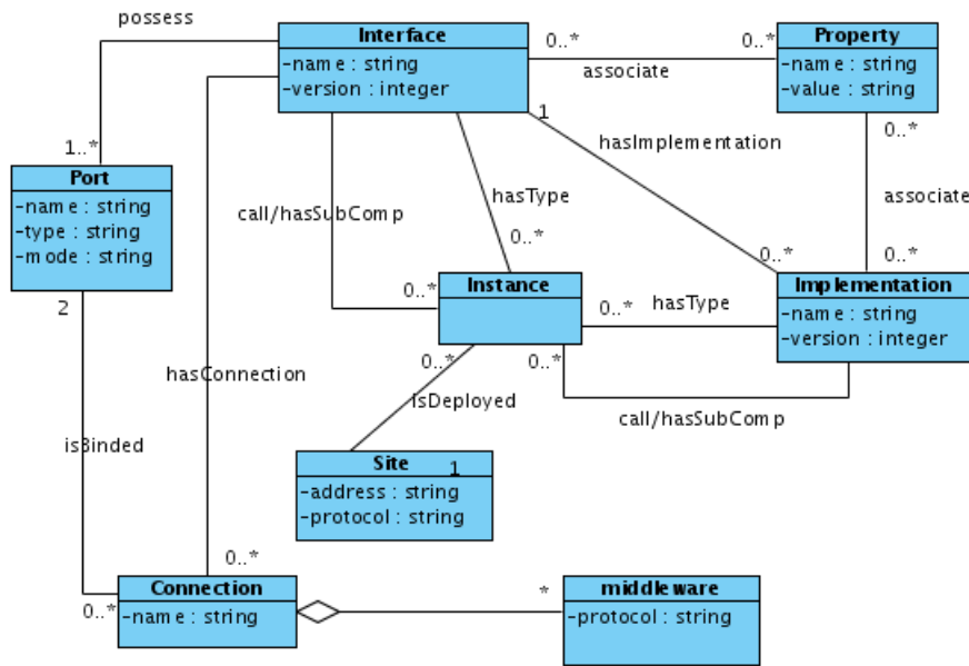
Figure 1: ASCM: UML-based representation of Architecture Description Languages
