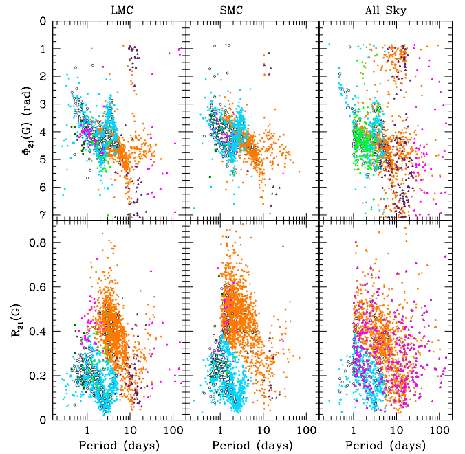
Fig. 37. Upper panels: G -band \phi_{21} vs. period diagram for Cepheids in the LMC (upper left), SMC (middle), and All-Sky (upper right). Lower panels: same as in the upper panels, but for the G -band R_{21} vs. period diagram. The symbols and colour-coding are the same as in Fig. 6.
