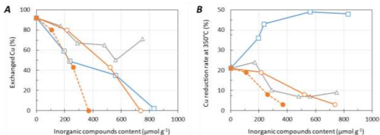
Figure 3. Exchanged copper distribution (A) and copper reduction rate up to 350 °C (B) in function of inorganic compounds content. (□, —): Cu/FER@(Na), ( \Delta , —): Cu/FER@(P), (○, —): Cu/FER@(Na+P); dotted lines (●, ---) correspond to data plotted depending on only Na or P contents ( [\text{Na}] = [\text{P}] ).
