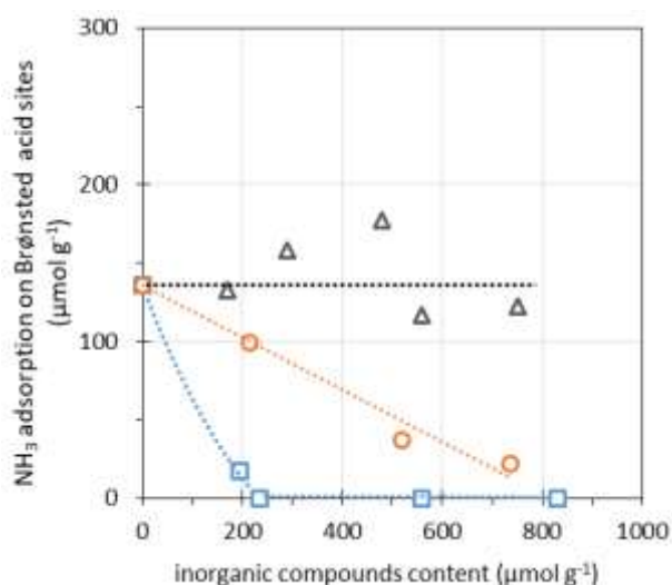
Figure 8. Ammonia adsorption capacities at 250°C from IR bands centered at 1452 and 1397 cm -1 , assumed to correspond only to the Brønsted acid sites of the zeolite. Influence of the mineral loading. (□, —): Cu/FER@Na, (△, —): Cu/FER@P, (○, —): Cu/FER@(Na+P);
