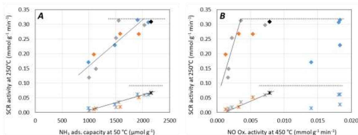
Figure 12. Relationship between standard (*) or fast (◆) SCR activities ( \text{mmol g}^{-1} \text{min}^{-1} ) at 250 °C in function of (A) NH 3 adsorption capacities at 50 °C ( \mu\text{mol g}^{-1} ) and (B) NO oxidation activities at 450 °C. (*, ◆): Cu/FeR; (*, ◆): Cu/FeR@Na; (*, ◆): Cu/FeR@P; (*, ◆): Cu/FeR@Na+P). In dotted line is presented the activity for 100 % NO x conversion in NH 3 -SCR.
