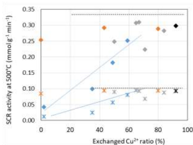
Figure 13. Relationship between standard (*) and fast (◆) SCR activities ( \text{mmol/g/min} ) at 500 °C in function of exchanged Cu 2+ ratio (%). (*, ◆): Cu/FeR; (*, ◆): Cu/FeR@Na; (*, ◆): Cu/FeR@P; (*, ◆): Cu/FeR@Na+P). In dotted line is presented the activity for 100 % NO x conversion in NH 3 -SCR.
