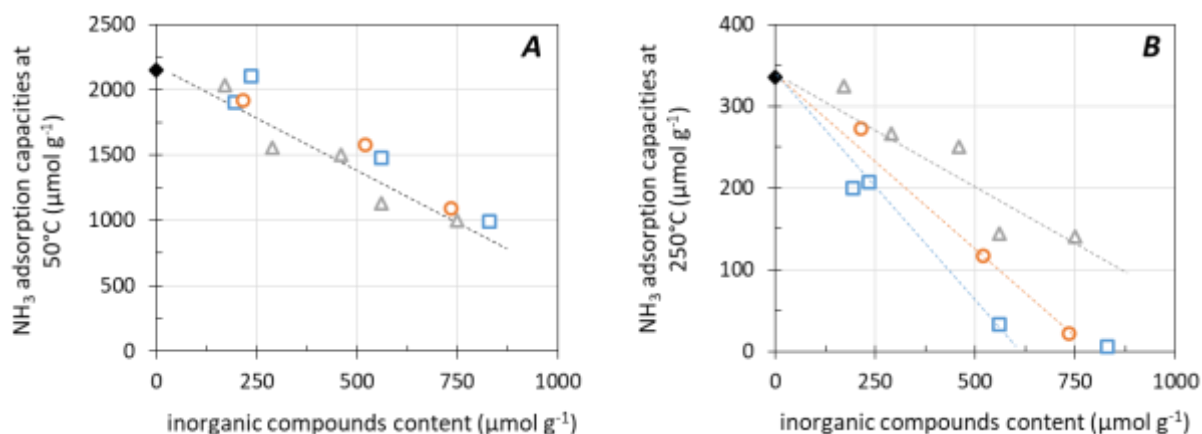
Figure 7. Effect of minerals addition on NH 3 adsorption capacities at (A): 50°C and (B): 250 °C (◆: Cu/FER; □: Cu/FER@Na; △: Cu/FER@P; ○: Cu/FER@(Na+P)).
