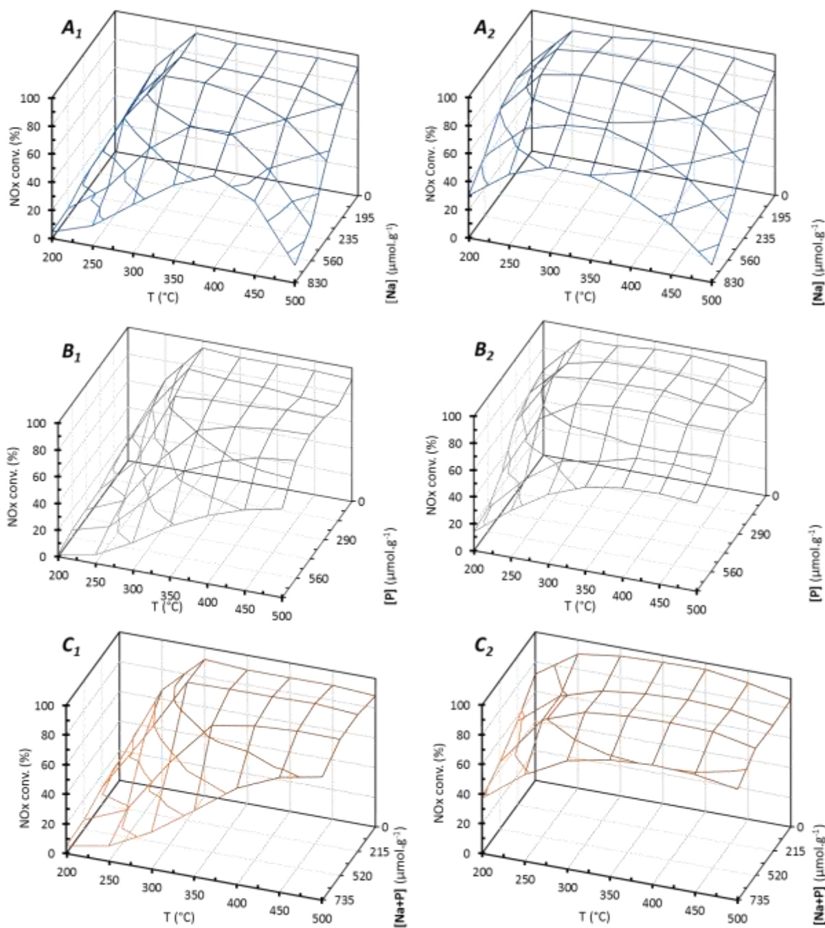
Figure 10. NH 3 -SCR performances in standard (1) and fast (2) condition in function of temperature and inorganic compounds content for (A): Na addition; (B): P addition; (C): Na+P addition. (—): Cu/FER@(Na), (—): Cu/FER@(P), (—): Cu/FER@(Na+P).
