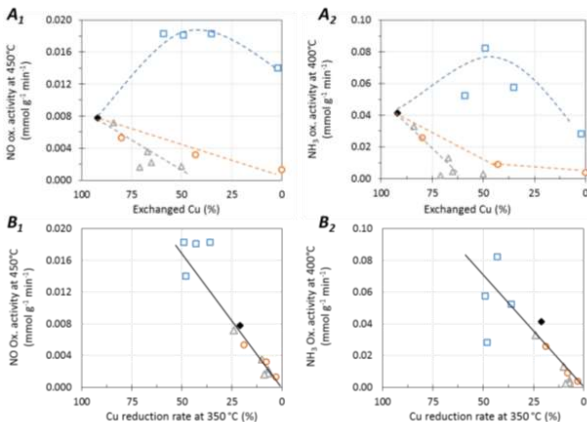
Figure 11. Effect of catalysts characteristics (exchanged \text{Cu}^{2+} ratio (A); copper reduction rate at 350°C from TPR profiles (B)) on NO and \text{NH}_3 oxidation activity. (◆: Cu/FER; □: Cu/FER@(Na); △: Cu/FER@(P); ○: Cu/FER@(Na+P)).
