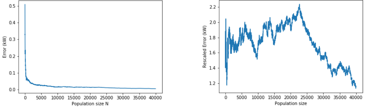
(a) Error \|\bar{v}^{(N)} - \bar{v}^{(\infty)}\|_{\mathcal{H}} as a function of population size N (conditionally to one scenario of P^{\text{sun}} )
