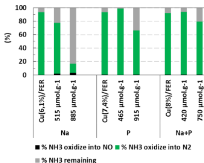
Fig. 4 Effect of Na, P and Na+P loading on NH 3 oxidation activities at 400°C
