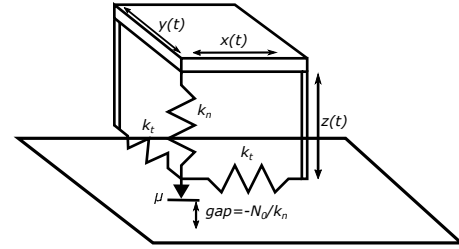
FIGURE 8: Contact model
