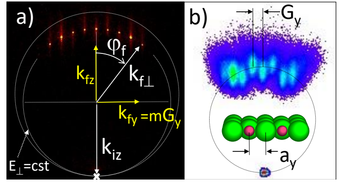
Fig. 4 a) Diffraction pattern of 300 eV He on LiF along the \langle 110 \rangle direction at \theta_f = 1.08^\circ ( k_{\perp} = 14.3 \text{ \AA}^{-1} ). The white cross indicates the location of the beam before target insertion. The line between this cross and the specular spot indicates the scattering plane k_{fy} = k_{iy} . The elastic diffraction spots fall on the Laue circle of energy conservation: k_{fy}^2 + k_{fz}^2 = k_{iz}^2 and exhibit diffraction along the y direction only k_{fy} = mG_y . b) early diffraction image from ref. 50 where elastic diffraction was not visible.
