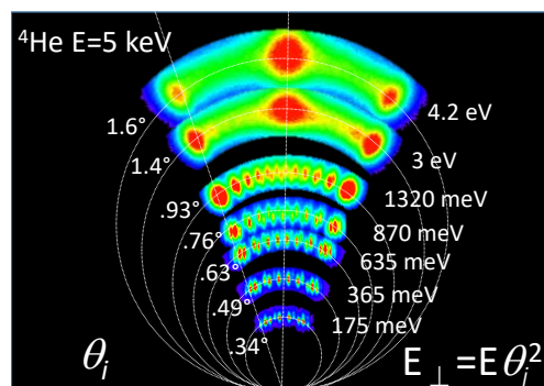
Fig. 15 Superposition of seven diffraction patterns measured with 5 keV ^4\text{He} projectiles on LiF aligned along the \langle 110 \rangle direction. The angle of incidence \theta_i is indicated on the left and the corresponding energy E_\perp on the right. All Bragg peaks can be resolved until E_\perp = 1.5\text{ eV} . Supernumerary rainbow structure (see text and fig.16) dominates above E_\perp = 300\text{ meV} . Above E_\perp = 2\text{ eV} only the Supernumerary rainbow structure persists but slowly weakens. At 4.2 eV only broad intensity variation persist as detail in fig.17.
