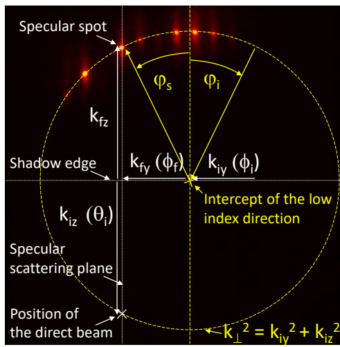
Fig. 9 Diffraction pattern of 460 eV He impinging along LiF \langle 110 \rangle with \theta_i = 0.9 deg. and an azimuth angle \phi_i = 0.45^\circ . The white dotted lines correspond to the intercept with macroscopic planes ; the horizontal shadow edge of the surface plane and its perpendicular the specular scattering plane which contains both the incident and specularly reflected projectiles. It corresponds to the impact of an effective particle with a momentum \hbar k_{\perp} = \hbar \sqrt{k_{iy}^2 + k_{iz}^2} with an incidence angle \phi_i = \arctan(k_{iy}/k_{iz}) \approx 26^\circ with respect to the surface normal.
