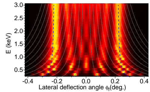
Fig. 8 diffraction charts of neon on LiF \langle 110 \rangle recorded at fixed incidence of 0.42 \text{ deg} and at incident energies between 300 eV and 3 keV. The energy E_{\perp} = E_0 \times 5.37 \cdot 10^{-5} .
