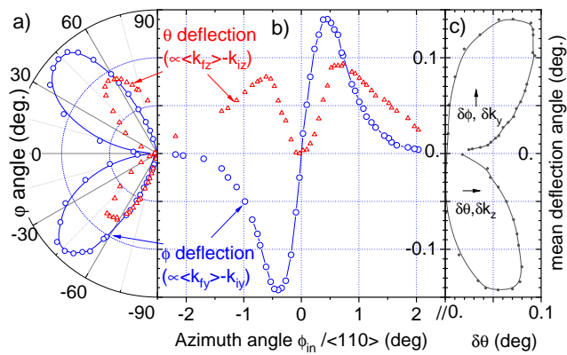
Fig. 13 For 460 eV helium on a LiF(001) surface at an incidence angle \theta=0.48^\circ and variable azimuth \phi_m , the mean lateral ( \phi_f ) and vertical ( \theta_f ) deflection referred to the specular beam are reported in three different forms. b) is a cartesian plot as a function of the azimuth angle \phi_m referred to \langle 110 \rangle direction 17 . a) is a polar plot as a function of the angle \phi_i = \arctan(k_{iy}/k_{iz}) . c) describes the trajectory of the mean impact position ( (\langle \theta_f \rangle, \langle \phi_f \rangle) ) as the incident azimuth \phi_i is varied.
