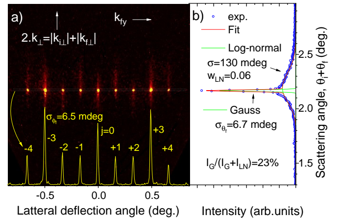
Fig. 5 Same as fig.4a) but the vertical axis is now k_{\perp eff} = |k_{\perp}| + |k_{f\perp}| corresponding to the diameter of the dotted circle going through the beam in fig.4a). The Laue circle is now a horizontal line and the intensity on a 6 mdeg wide horizontal band is reported in yellow at the bottom. b) The projection of a) on the vertical axis gives the polar scattering distribution P(\theta_f) . It indicates two components, a narrow quasi-gaussian and a much broader one having a quasi-log-normal profile.
