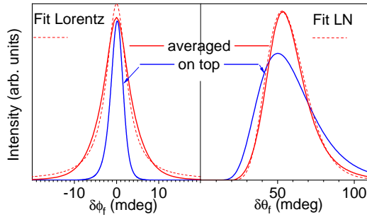
Fig. 24 Angular straggling \sigma\theta_f (right) and \sigma\phi_f (left) of an individual inelastic collision averaged over the lattice cell 18 . Compared with the "on-top" trajectory, the lateral broadening has acquired a partial Lorentzian character while the log-normal scale parameter w \sim \sigma\phi_f/\theta_s describing the broadening of the polar distribution is reduced by \approx 30\% .
