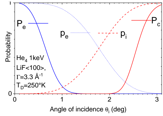
Fig. 22 The probability p_e and P_e = \Pi_1^{N_{eff}} p_e of individual and overall elastic scattering respectively. The complementary inelastic probabilities p_i = (1 - p_e) and P_c = \Pi_1^{N_{eff}} p_i are plotted as a function of the angle of incidence \theta_i for 1 keV He.
