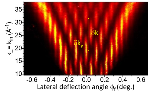
Fig. 7 diffraction charts of 500 eV neon on LiF \langle 110 \rangle recorded at incidence angles \theta_i between 0.25 and 1 deg. corresponding to E_{\perp} = 9.5 and 76 \text{ meV} respectively. In the paraxial region, a pseudo period is observed \delta k_{\perp} \sim 13.3 \text{ \AA}^{-1} and \delta k_y \sim 2G_y .
