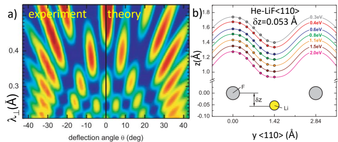
Fig. 14 a) Comparison of experimental and calculated diffraction chart of He on LiF along \langle 110 \rangle as a function of the wavelength \lambda_\perp . b) The calculated potential energy landscape and, in the bottom the atomic positions highlighting the rumpling by 0.053\text{\AA} of the \text{Li}^+ ions.
