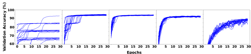
(a) Dropout : 0%
