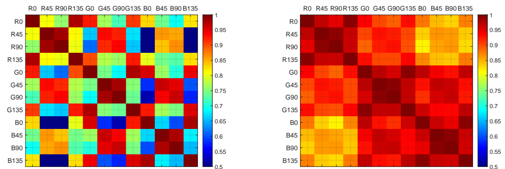
Figure 5. (a) Total Scene and (b) Total \ {Active} Scene correlation coefficients tables shown in false colors.
