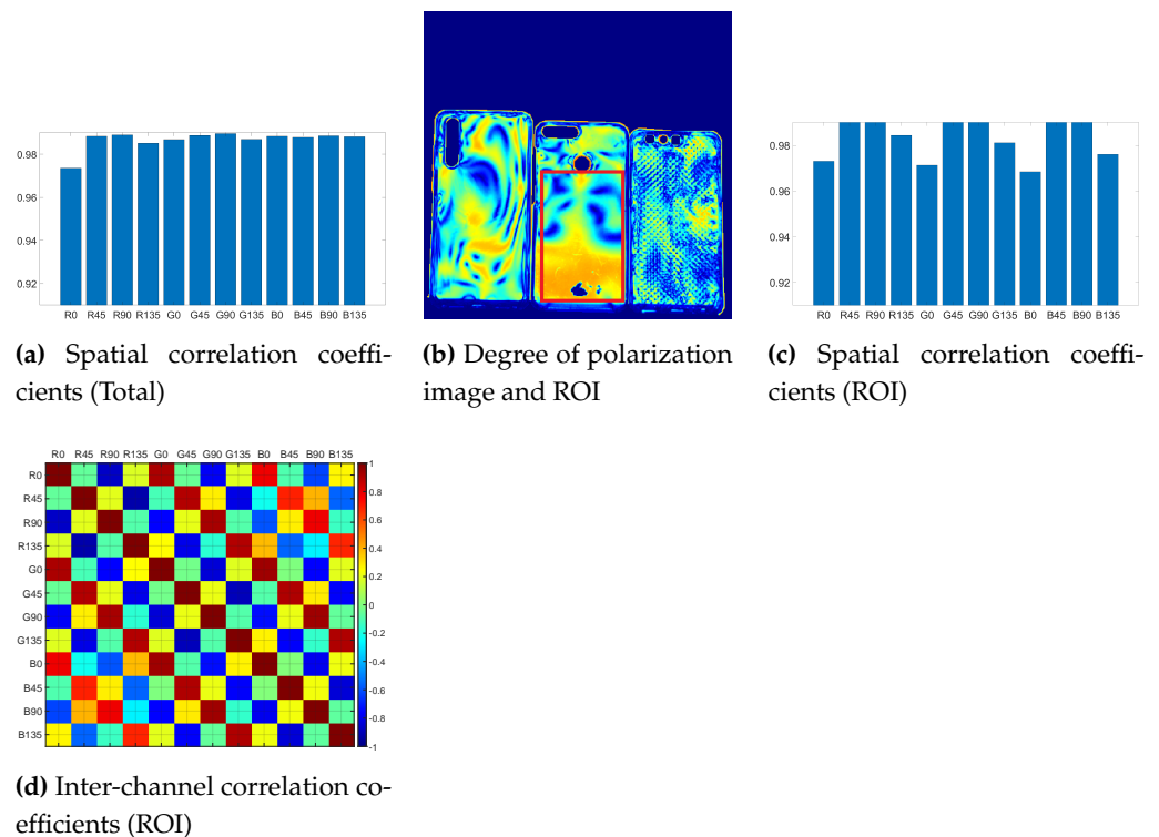
Figure 6. (a) Spatial correlation coefficients computed for all of the observations. (c) Spatial correlation coefficient computed from an active polarization scene (“cellphonecases” scene in Figure 2h), where the Region Of Interest (ROI) selected is surrounded in red in (b). (d) Inter-channel correlation coefficients computed for the ROI.
