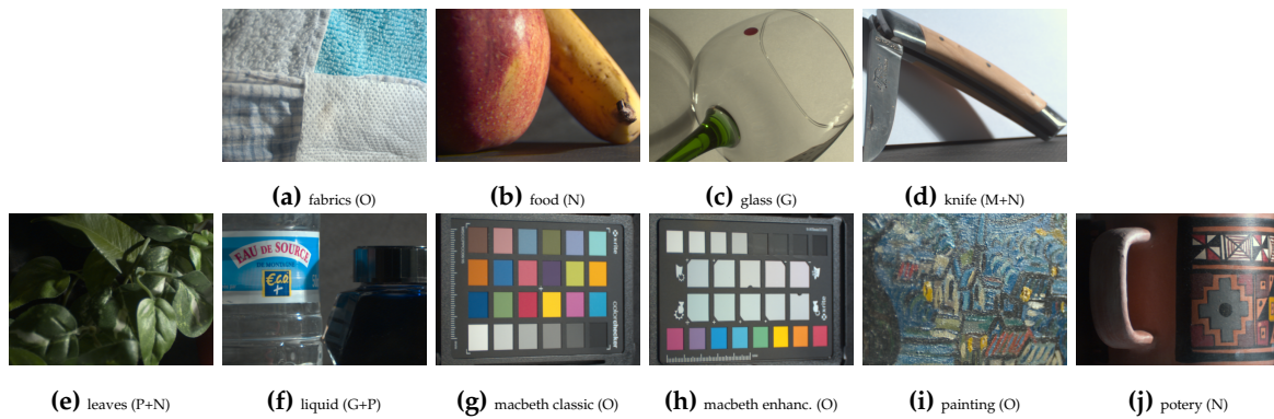
Figure 3. Visualization of the 10 scenes of the data from Lapray et al. [32] by alphabetical order. The material clustering for each scene is represented by the acronym: M (Metallic), N (Natural), A (Active), P (Plastic), G (Glass), and O (Other).
