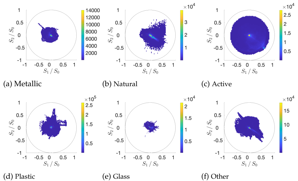
Figure 4. Scatter plots of polarization data for material clusters for the green channel ( c = G ), approximating the luminance. We also observe similar behaviors on the red and blue channel. Each plot represents the plane of the equator of the Poincaré sphere (latitude is zero for linear polarization). The Stokes component values [25] S_1 = \rho_{0,G} - \rho_{90,G} and S_2 = \rho_{45,G} - \rho_{135,G} are normalized with respect to the total irradiance S_0 = \rho_{0,G} + \rho_{90,G} . The center of the circle represents unpolarized data, whereas the unit circle represents fully polarized data. The distance from the center is the degree of linear polarization DOLP = \frac{\sqrt{S_1^2 + S_2^2}}{S_0} , and the angle with respect to the origin is 2\beta , so that the orthogonal polarizations are shown to be diametrically opposed.
