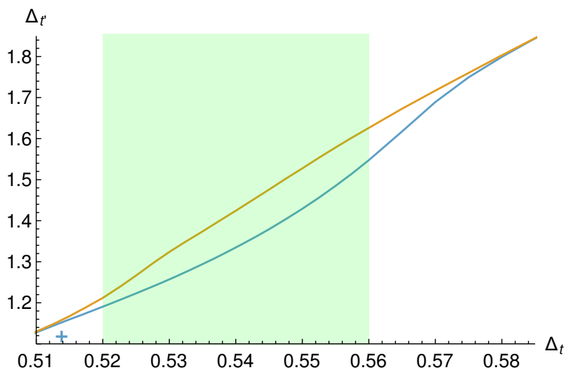
Figure 13: The blue line shows the bound on the dimension of the first traceless symmetric operator exchanged in the t \times t OPE. The orange line shows the bound on the dimension of the first additional traceless symmetric operator t' when assuming the exchange of t itself. The blue cross indicates the large N estimate of the position of the O(9) model. The green region shows the prediction for the ARP^3 model from lattice computations. In the ARP^3 region allowing the exchange of t itself lifts (weakens) the bound. The two lines join again at a third kink outside the expected ARP^3 region. The bounds have been obtained at \Lambda = 27 .
