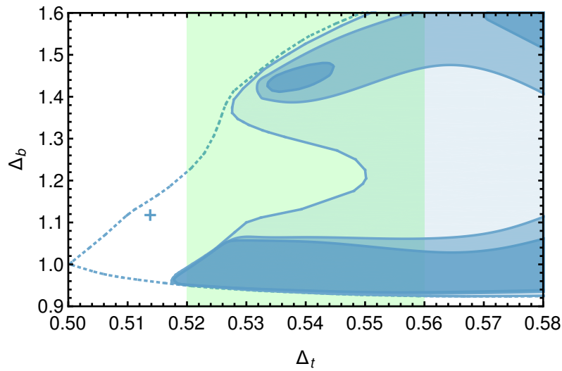
Figure 22: Allowed region in the (\Delta_t, \Delta_b) plane assuming the existence of exactly one relevant Box scalar and \Delta_{T'} > 4.5 , \Delta_{J'} > 3 and \Delta_h > 2.05 . The green region shows the prediction for the ARP^3 model from lattice computations. The bounds have been obtained at \Lambda = 19, 27, 31 (light to dark). The isolated island disappears when we push to \Lambda = 35 , indicating that at least one of these assumptions is too strong. The dashed line indicates the allowed region assuming only the existence of exactly one relevant Box scalar without additional assumptions.
