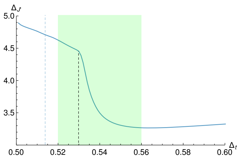
Figure 11: Bound on the dimension of the first spin-1 antisymmetric vector after the conserved current. The blue dashed line indicates the large N estimate of \Delta_\phi for the O(9) model. The green region shows the prediction for the ARP^3 model from lattice computations. We see a clear kink within this region indicated by a black dashed line. In addition, various small kinks or wobbles appear in the region 0.51 < \Delta_t < 0.52 though not in correspondence with large N estimate of the location of the O(9) model. The bounds have been obtained at \Lambda = 27 .
