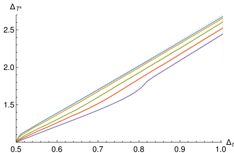
Figure 7: Bound on the dimension of the first four-index-symmetric scalar. The blue, orange, green, red and purple lines correspond respectively to N = 4, 5, 10, 20, 100 . Apart from a kink at the location of the O(N') model few features are visible. At N = 100 an additional kink becomes visible. These bounds have been obtained at \Lambda = 27 . The dotted lines indicate the same bound at \Lambda = 19 and are included to illustrate the convergence. The bounds get strictly stronger for larger N .
