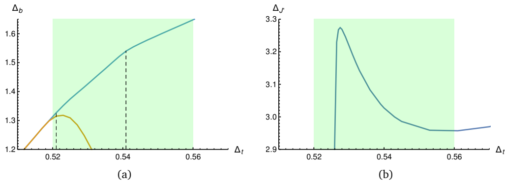
Figure 19: On the left: Bound on the dimension of the first scalar Box operator. The blue line shows the bound under no assumptions while the orange line is found under the assumptions \Delta_{T'} > 5.5 and \Delta_{J'} > 3 . The orange line shows a maximum close to the position of the first kink of the blue line. The green region shows the prediction for the ARP^3 model from lattice computations. These bounds were obtained at \Lambda = 19 On the right: The bound on the first antisymmetric spin-1 operator after the conserved current assuming \Delta_{T'} > 4.5 , \Delta_h > 2.05 and \Delta_b > 1.37 . This bound has been obtained at \Lambda = 35 .
