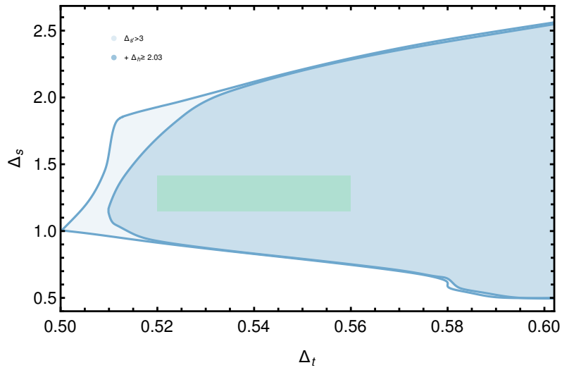
Figure 24: Allowed region in the (\Delta_t, \Delta_s) plane assuming the existence of exactly one relevant singlet and \Delta_h > 2.03 . The green region shows the prediction for the ARP^3 model from lattice computations. The bounds have been obtained at \Lambda = 19 .
