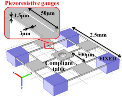
Figure 1. Illustration of the multi-axis piezoresistive MEMS force sensor
