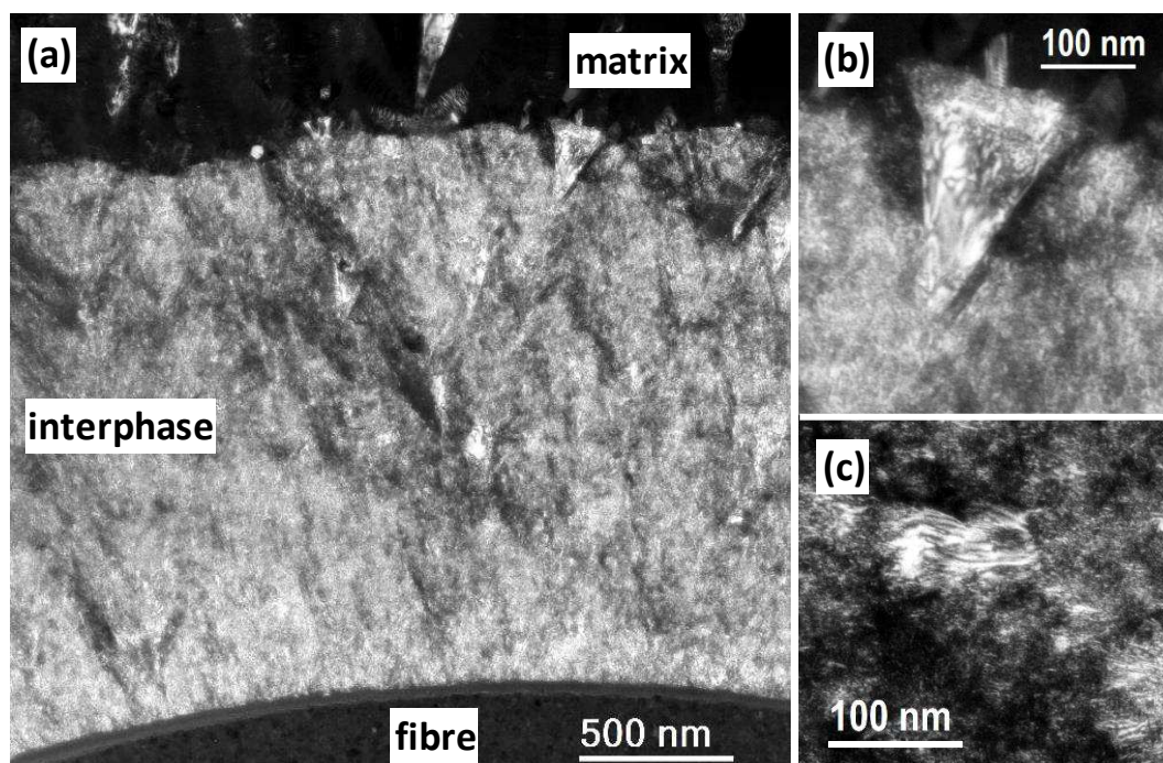
Fig. 2. (a) DF images of a BN interphase synthesized at 1200 °C with H 2 (12/H/T sample), enlarged images of (b) a crystallite of triangular shape and (c) a plate-like crystallite
