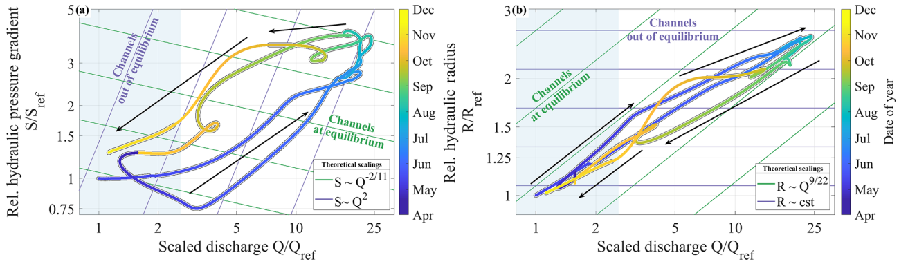
Figure 10. (a) Relative hydraulic pressure gradient \frac{S}{S_{ref}} and (b) hydraulic radius \frac{R}{R_{ref}} as inverted from seismic observations and as shown as a function of measured relative water discharge \frac{Q}{Q_{ref}} . Time series of R and S are calculated from 5 d low-pass-filtered time series of Q and P_w and are then 30 d low-pass-filtered (same as in Fig. 8). Time series of Q is 30 d low-pass-filtered. Reference values for all three variables are taken as the first day of the 2017 melt season (10 May 2017). We compare our data to the predictions of Röthlisberger (1972) for subglacial channels evolving at equilibrium with Q (green lines; S \propto Q^{-2/11} and R \propto Q^{9/22} ) and for subglacial channels evolving through hydraulic pressure gradient changes only (blue lines; S \propto Q^2 and \frac{\partial R}{\partial Q} = 0 ). Arrows show the direction of time. Blue shaded areas represent the period when Q is lower than 1 \text{ m}^3 \text{ s}^{-1} . Line sections without the black edges show interpolated values of R and S using a cubic spline interpolation, as in Fig. 8.
