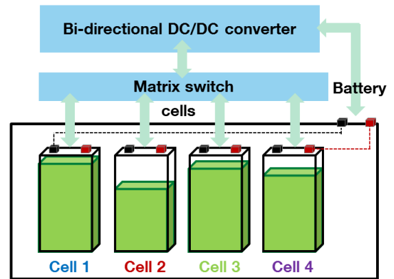
FIGURE 20. BMS architecture.
