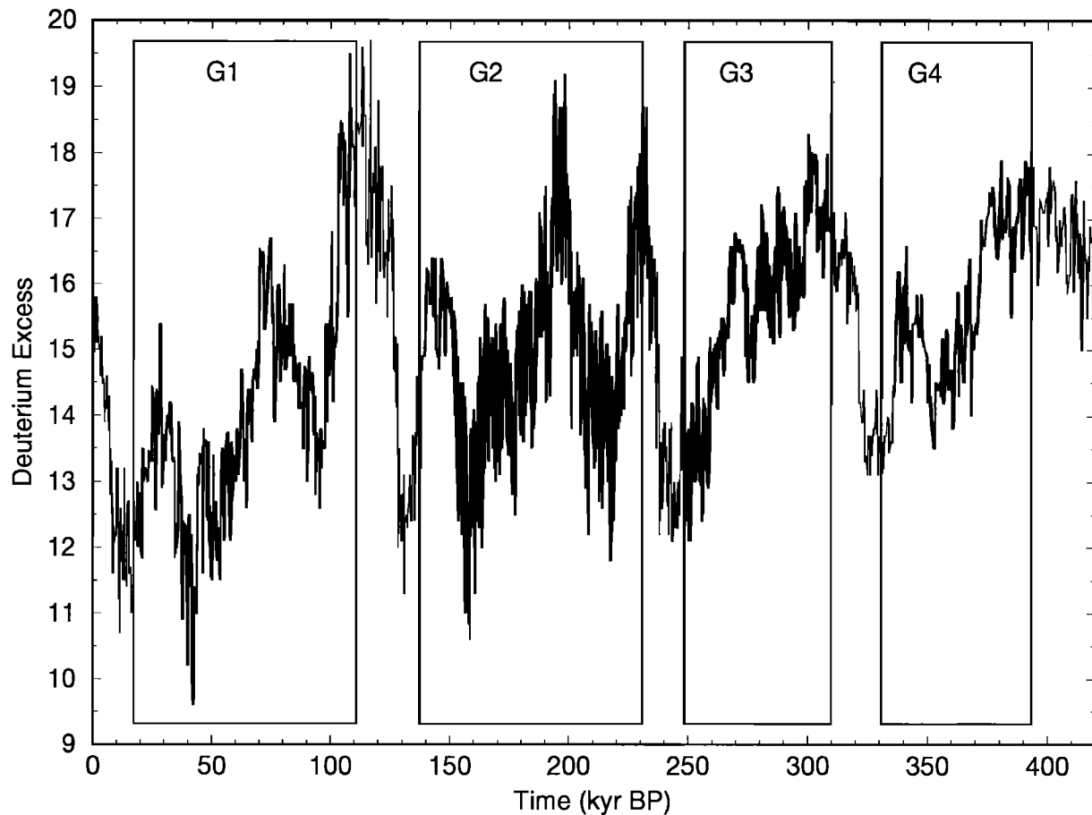
Figure 2. Deuterium excess d variations in the Vostok ice core. The four ice ages G1–4 are emphasized by boxes.
