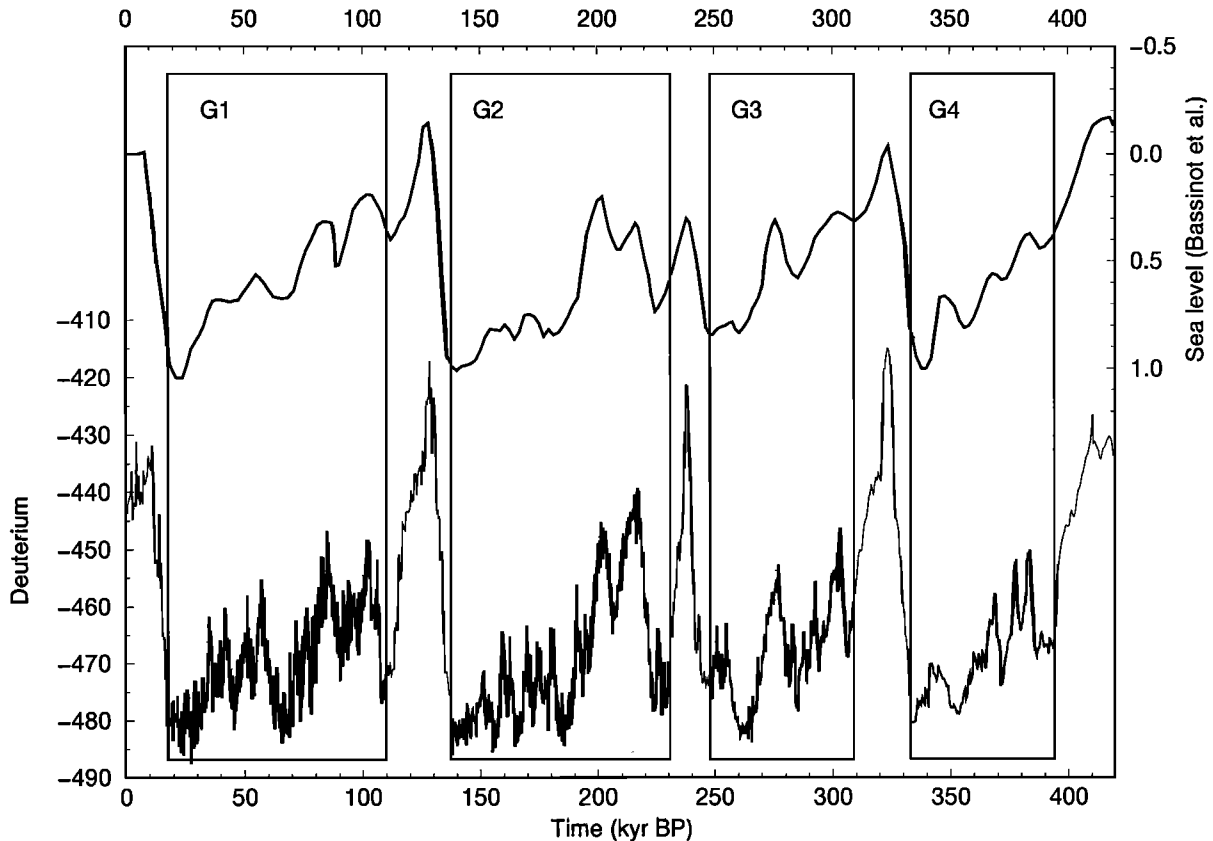
Figure 1. Deuterium \delta D variations in the Vostok ice core for the top 3305 meters. Time is expressed in thousands of years before present (kyr B.P.). Deuterium values are normalized by SMOW and expressed in per mil. The four ice ages are numbered from G1 to G4, and emphasized by boxes. The upper panel shows the sea-level change curve from the Bassinot et al. [1994] data.
