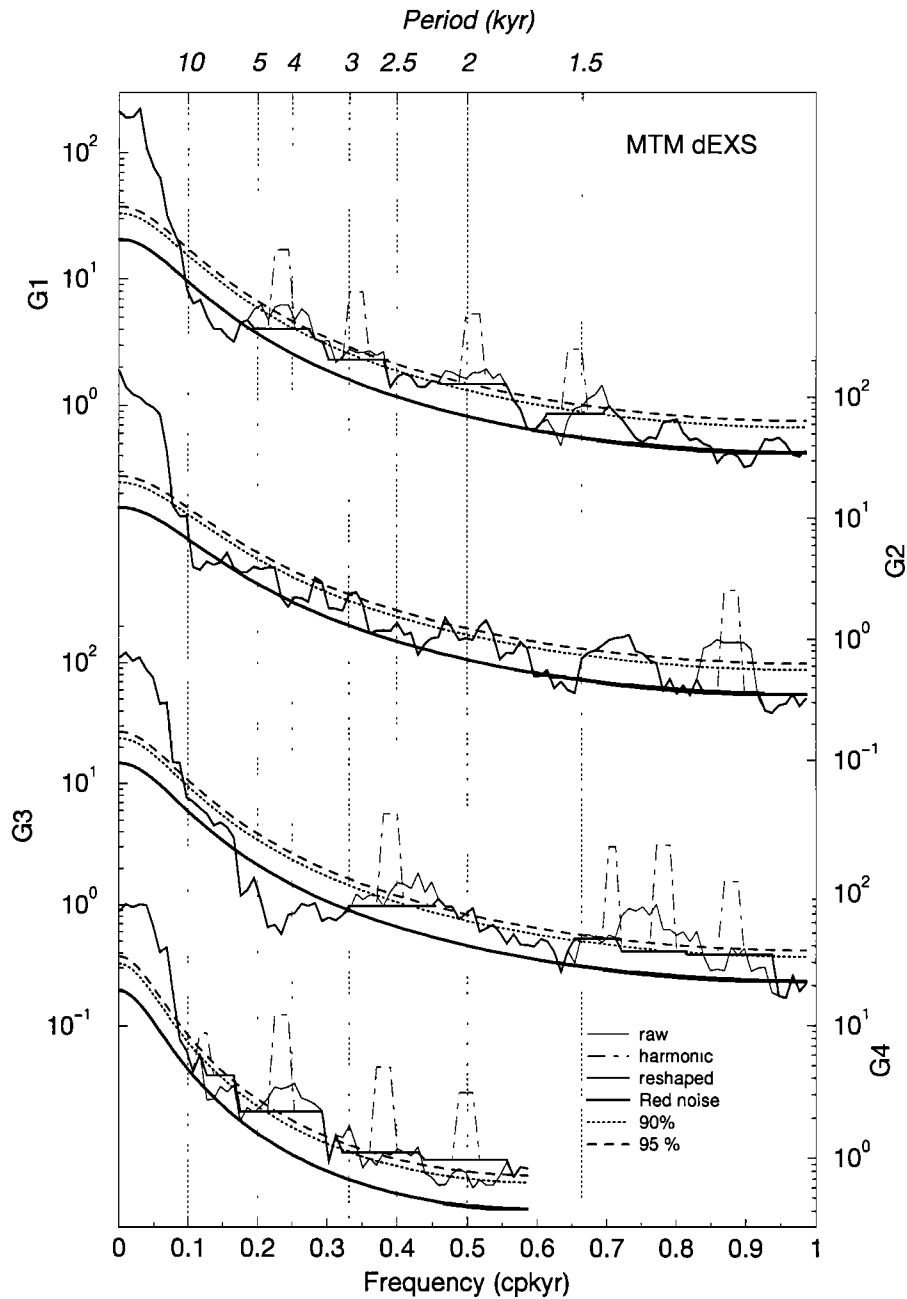
Figure 4. MTM spectral analyses of the four glacial d records (G1–4 from top to bottom, respectively). The MTM parameters are a NW = 4 bandwidth and K = 7 tapers. The legends are the same as for Figure 3.
