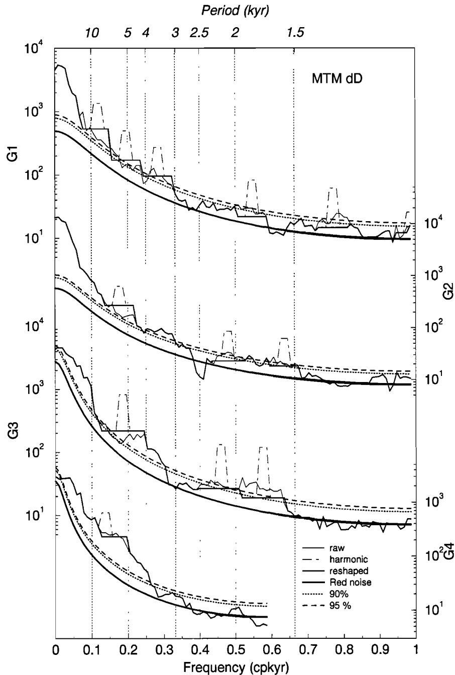
Figure 3. MTM spectral analyses of the four glacial \delta D records. The four ice ages G1–4 go from top to bottom. The G4 spectrum is truncated at 0.6 cycles/kyr because of its poorer resolution. The MTM parameters are a NW = 4 bandwidth and K = 7 tapers (see Yiou et al. [1996] for methodological details). The thin wiggly lines represent the raw spectra; the thin dash-dotted lines, the harmonic peaks detected by the F -test [ Mann and Lees , 1996]; the thick wiggly line, the reshaped spectra, after removal of the harmonic components [ Thomson , 1982; Mann and Lees , 1996]; the thick continuous line is the equivalent red noise spectrum obtained by robust median testing [ Mann and Lees , 1996]; the dotted and dashed lines are the 90% and 95% confidence intervals for the red noise null hypothesis.
