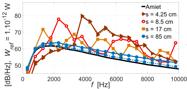
Figure 9: Downstream sound power spectra obtained from CAA with various channel widths s . Fine meshes (for the cases s = 4.25 cm and s = 85 cm) in dashed lines.
