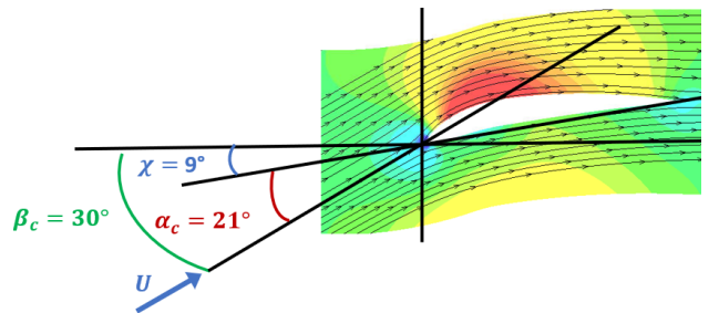
Figure 4: u'_x [ \text{m}\cdot\text{s}^{-1} ] (levels between 60 and 120).
