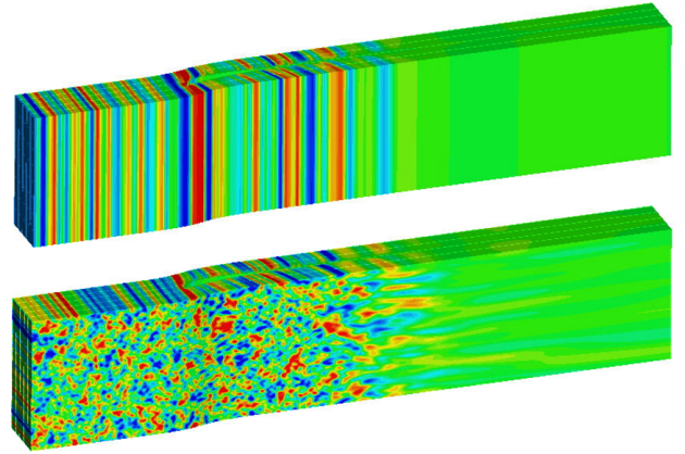
Figure 6: Snapshots of u'_y [ \text{m}\cdot\text{s}^{-1} ] for the parallel (top) and oblique (bottom) gusts (levels between -2 and 2).
