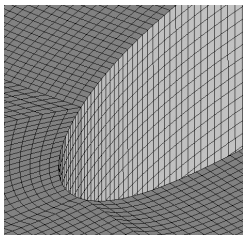
Figure 3: CAA mesh at the leading edge.
