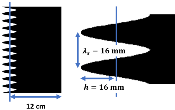
Figure 16: Geometrical parameters of the serrated design.
