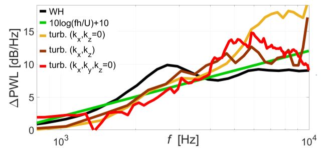
Figure 23: Downstream noise reduction for different synthetic turbulences. Analytical noise reduction coming from the Wiener-Hopf technique and law 10 \log(fh/U) + 10 .
