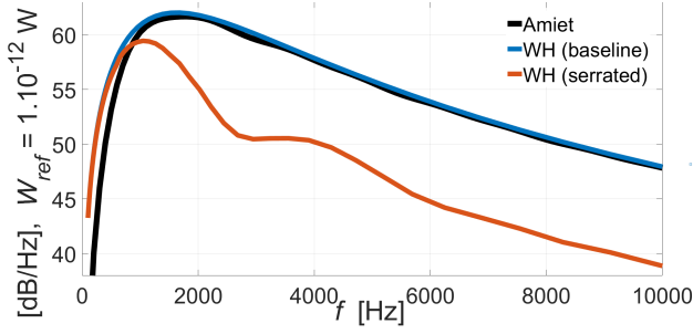
Figure 19: Downstream sound power for an isolated flat plate with Amiet and the Wiener-Hopf technique.
