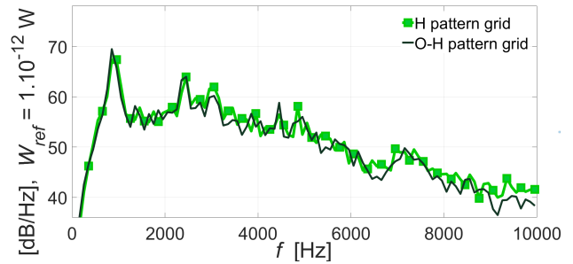
Figure 18: Downstream sound power per vane of a 3 channels computation (baseline geometry) for the H and O-H pattern meshes. Averaging over 100 Hz bands.
