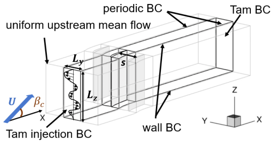
Figure 2: CAA set-up used for the simulation.
