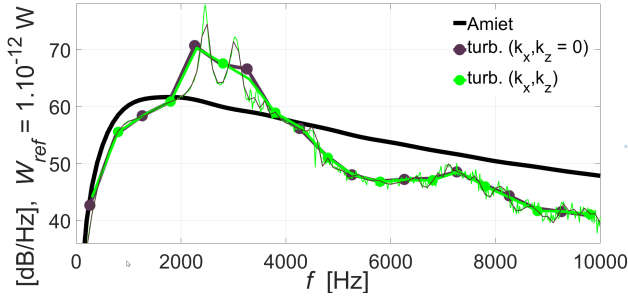
Figure 7: Downstream sound power obtained from numerical predictions and Amiet theory (isolated flat plate). Raw spectra in dashed lines and averaged (500 Hz bands) in solid lines.
