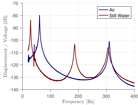
Fig. 6. In-air and in-water frequency response functions of the cantilever plate.
